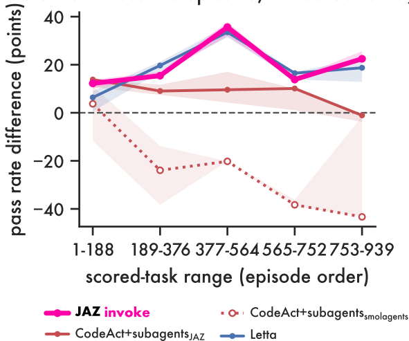
StuLife across the episode, minus CodeAct
