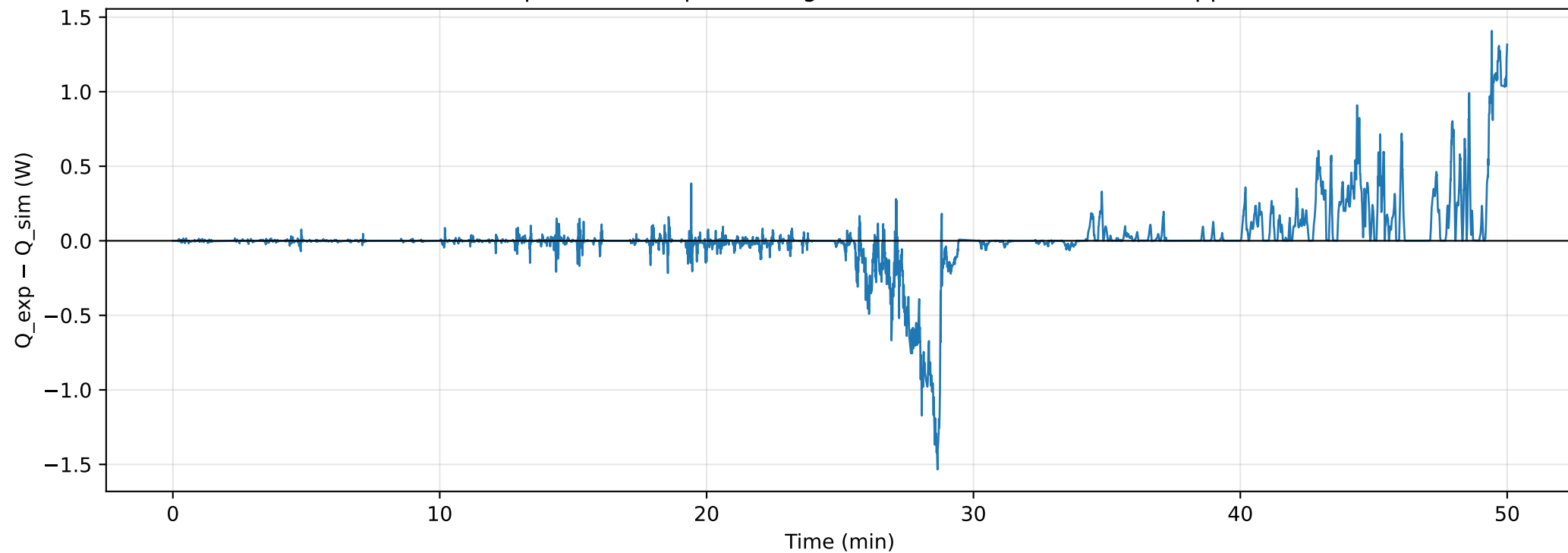
Residual (positive = experiment generates more heat than sim applies)
