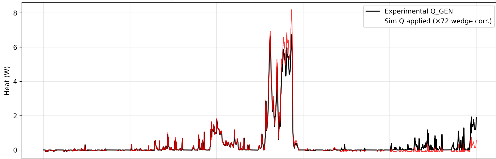
Heat generation: sim vs experiment (RMSE = 0.186 W)
