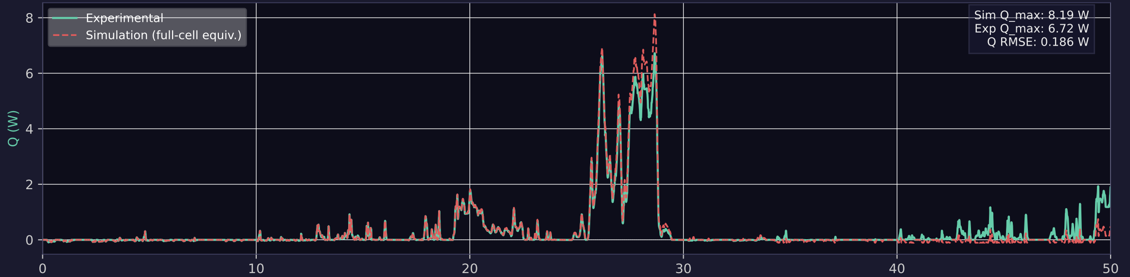
Heat Generation 0-3000 s
