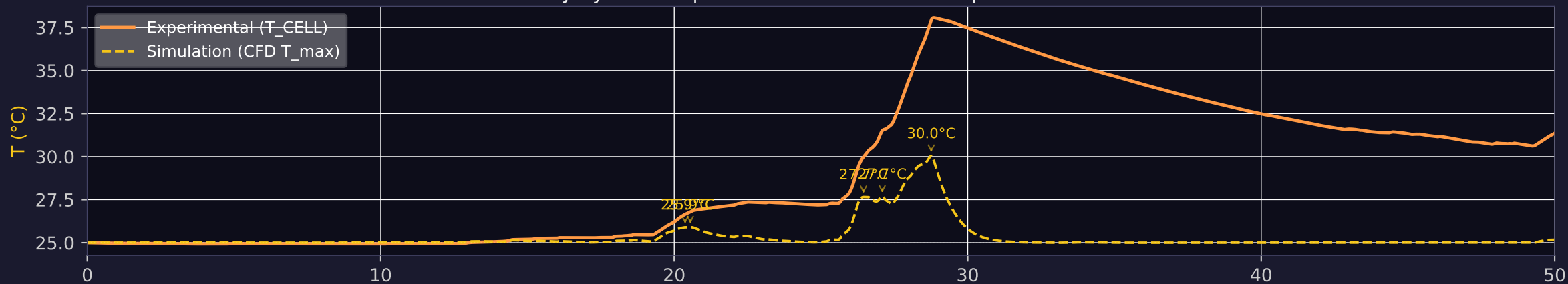
Jelly-Roll Temperature — Simulation vs Experimental
