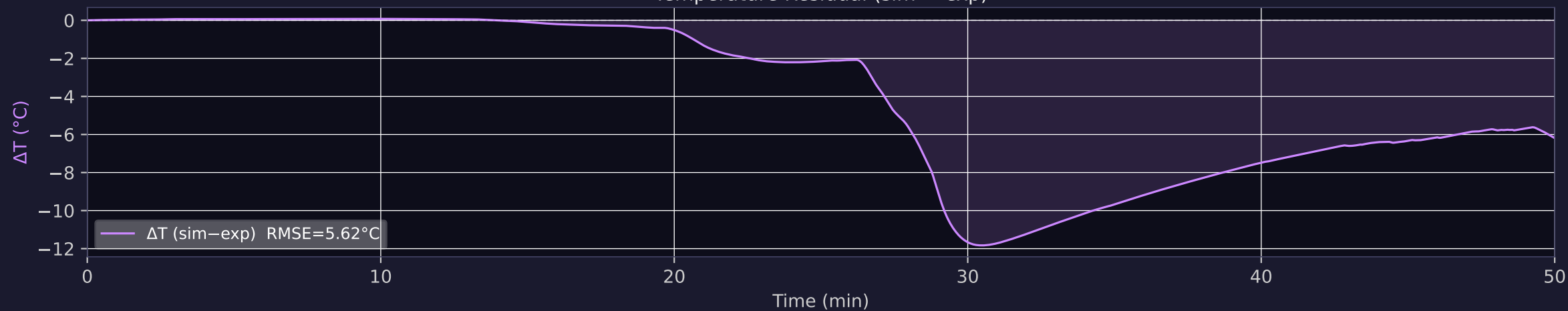
Temperature Residual (sim – exp)
