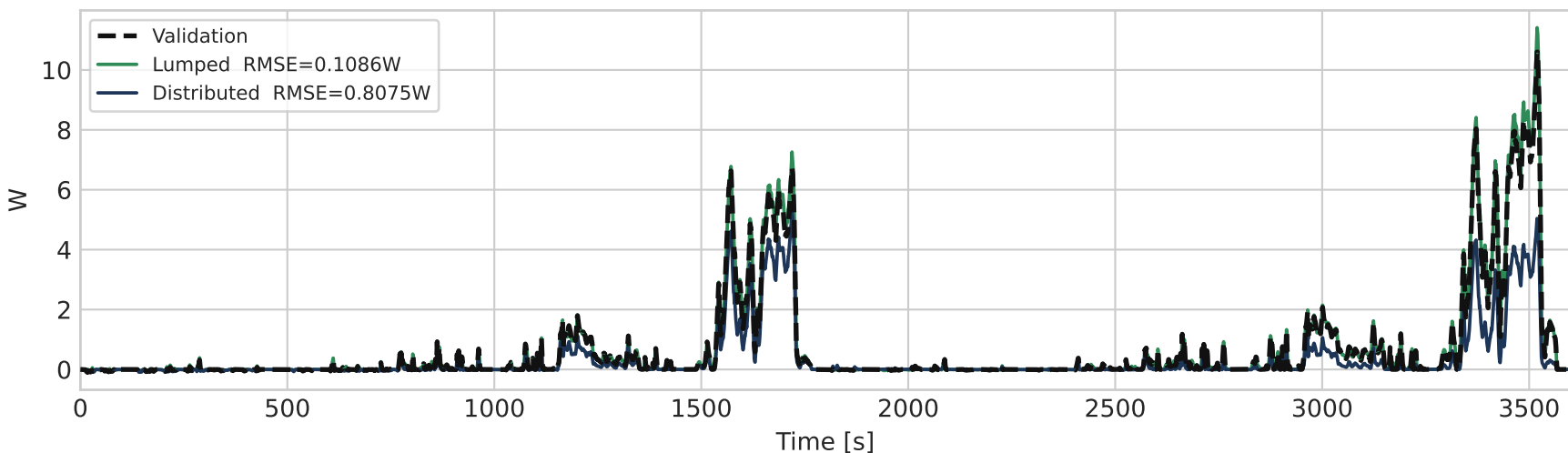
Heat Generation Q [W]
