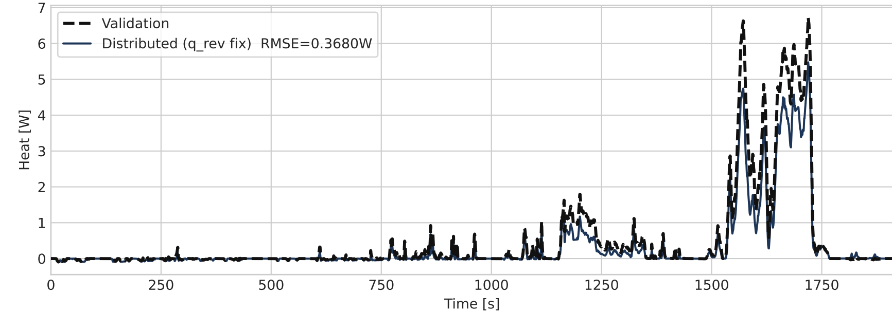
Heat Generation
