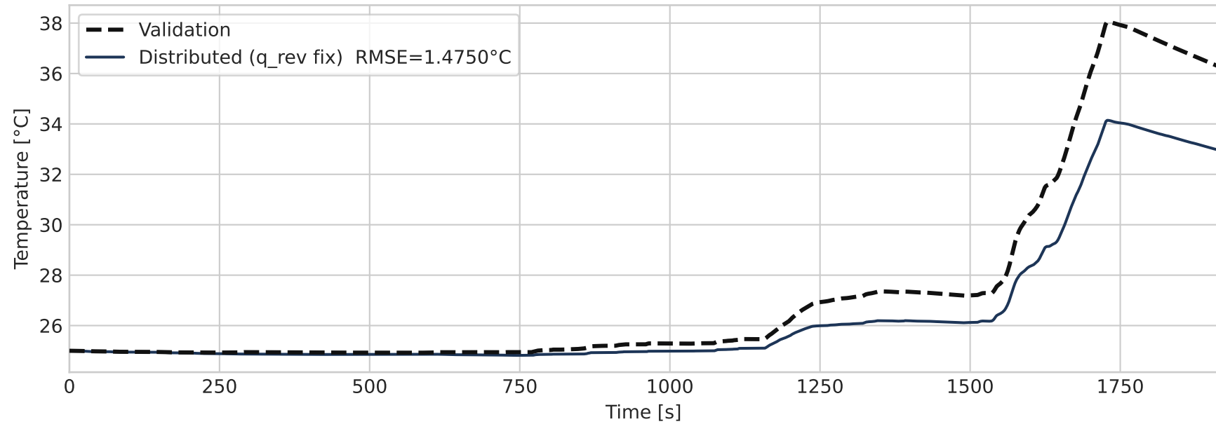
Cell Temperature
