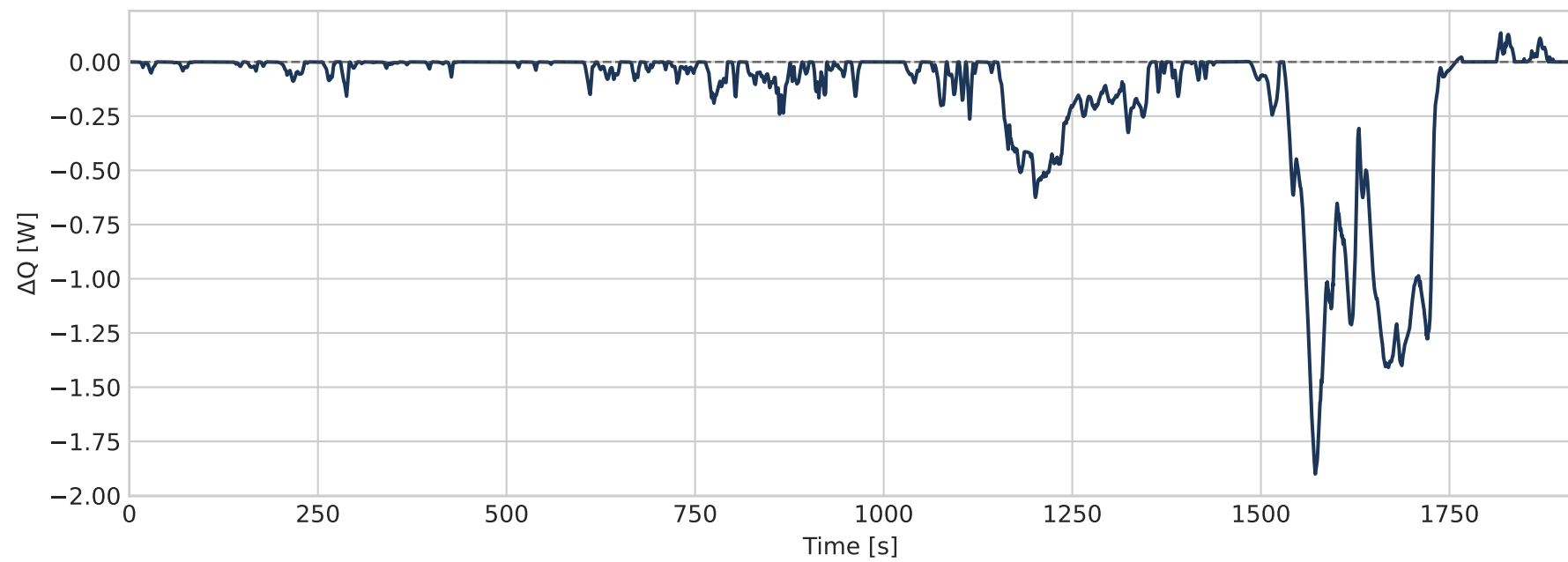
Heat Error: Model — Validation
