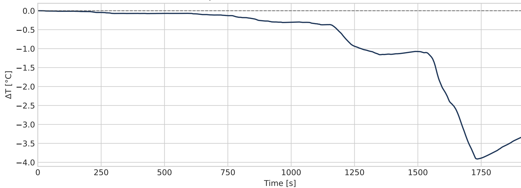
Temperature Error: Model — Validation
