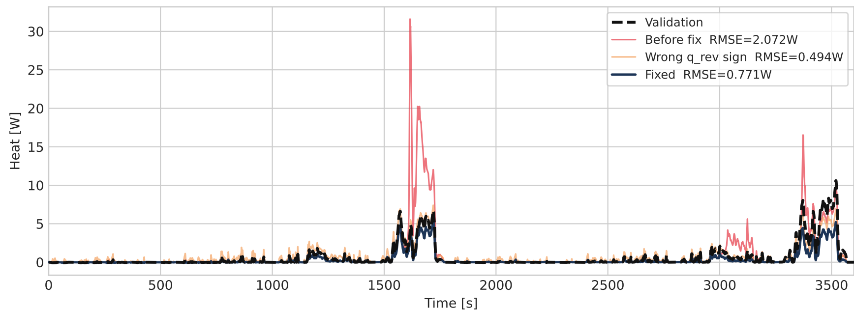
Heat Generation
