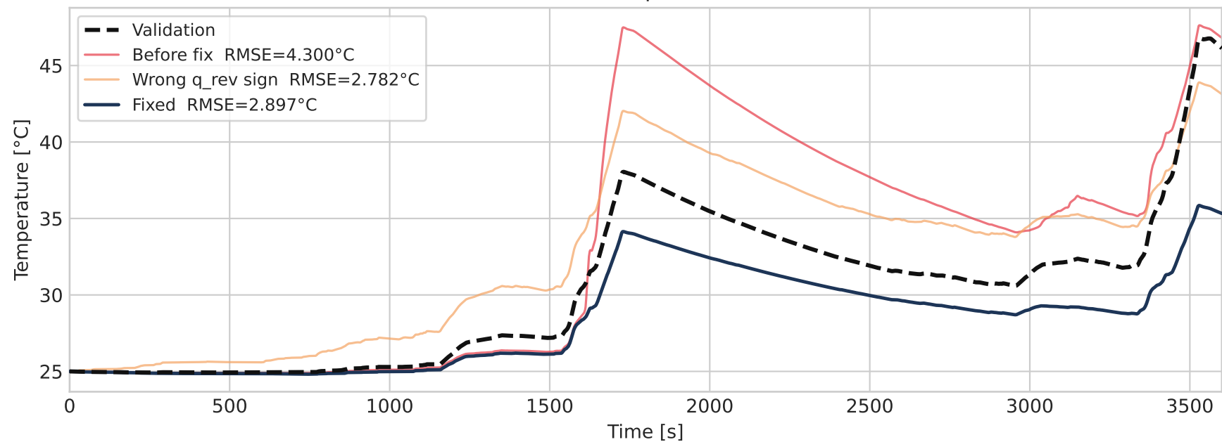
Cell Temperature
