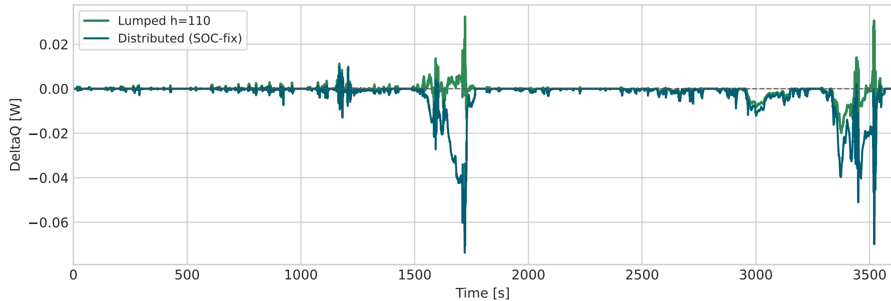
Heat Generation Error: Model - Validation
