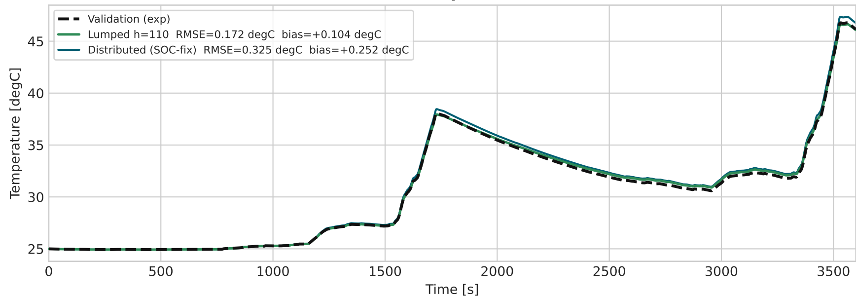
Cell Temperature
