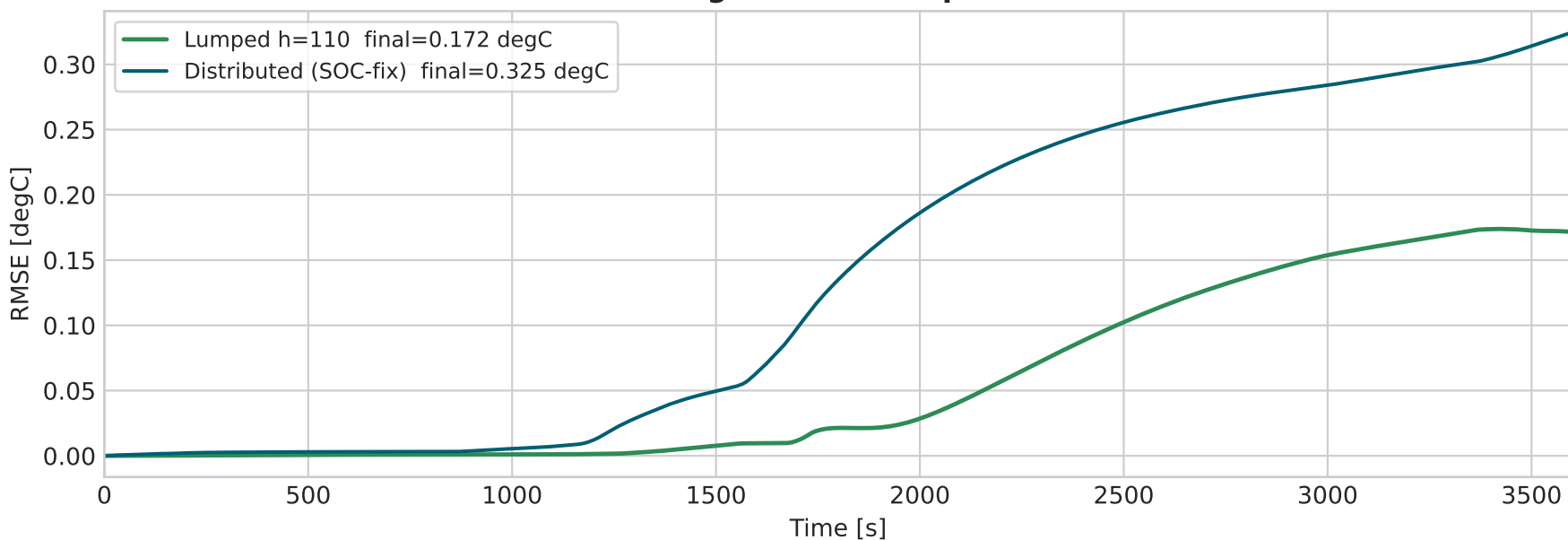
Running RMSE — Temperature
