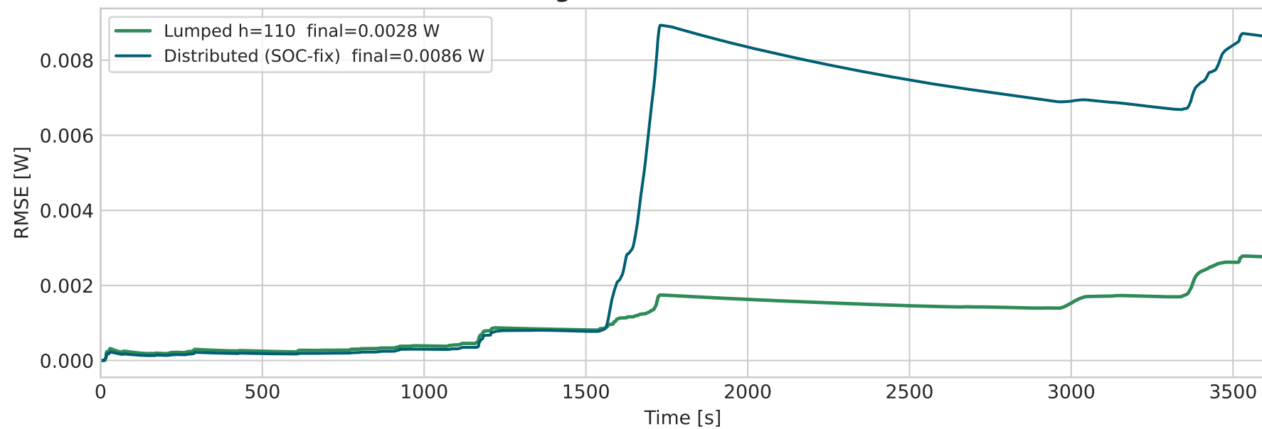
Running RMSE — Heat Generation
