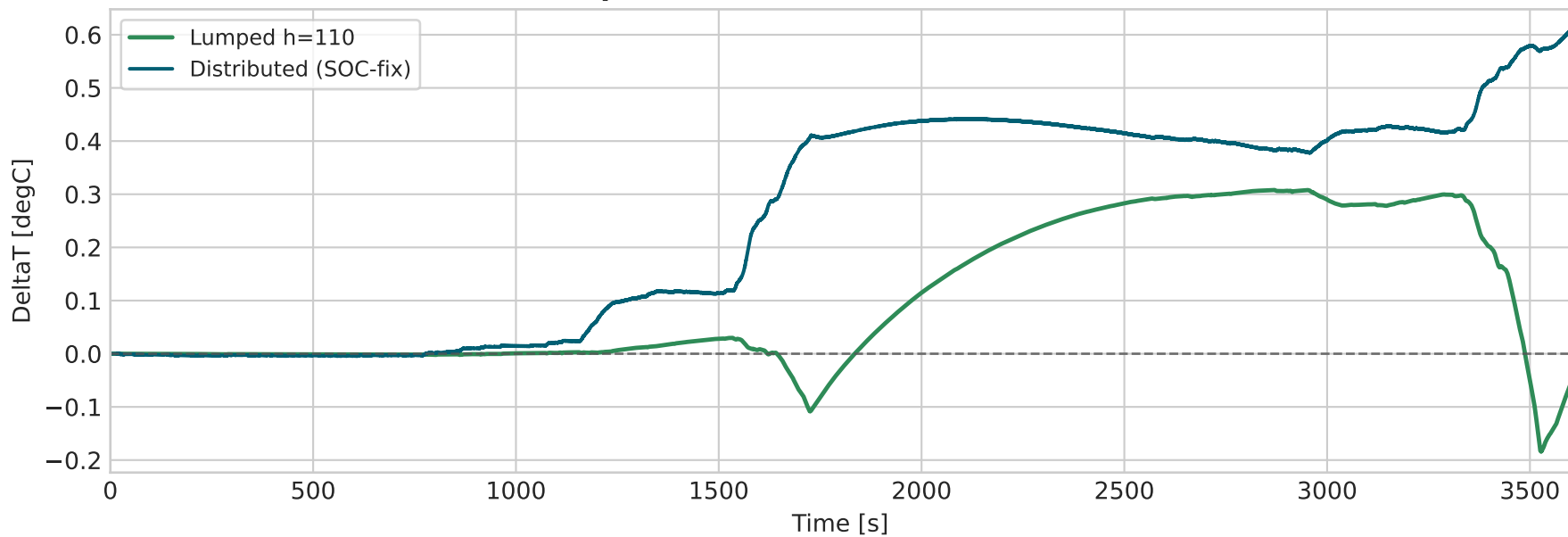
Temperature Error: Model - Validation
