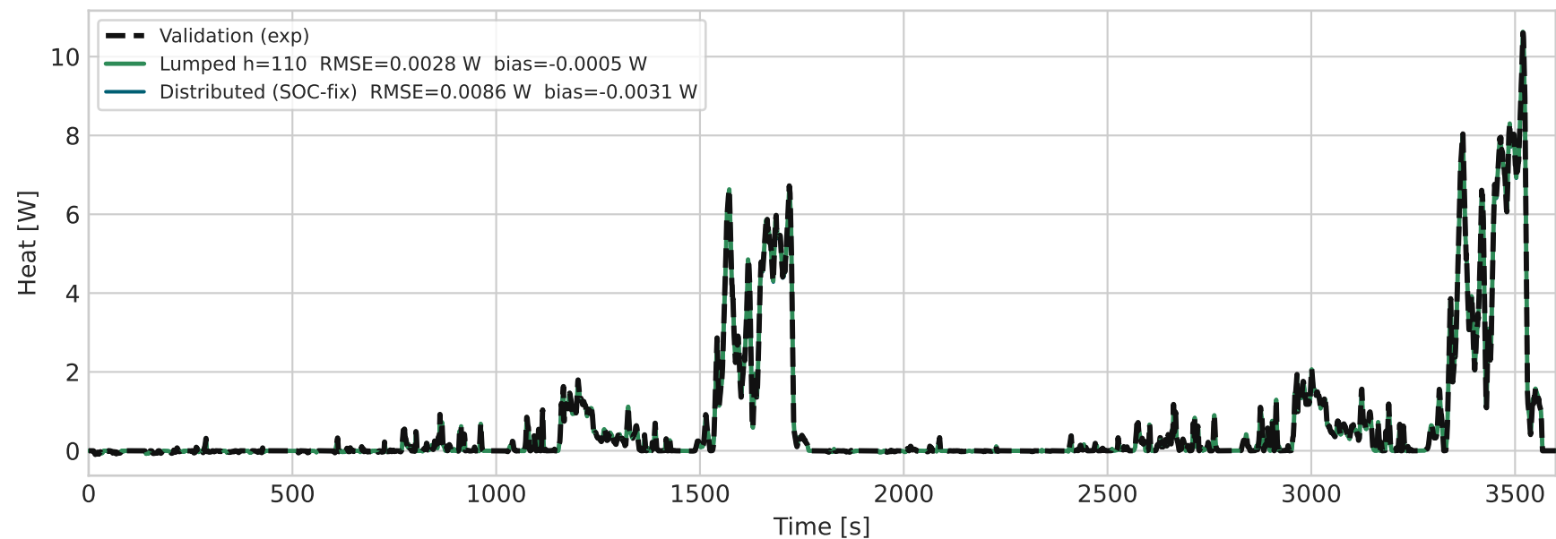
ECM Heat Generation
