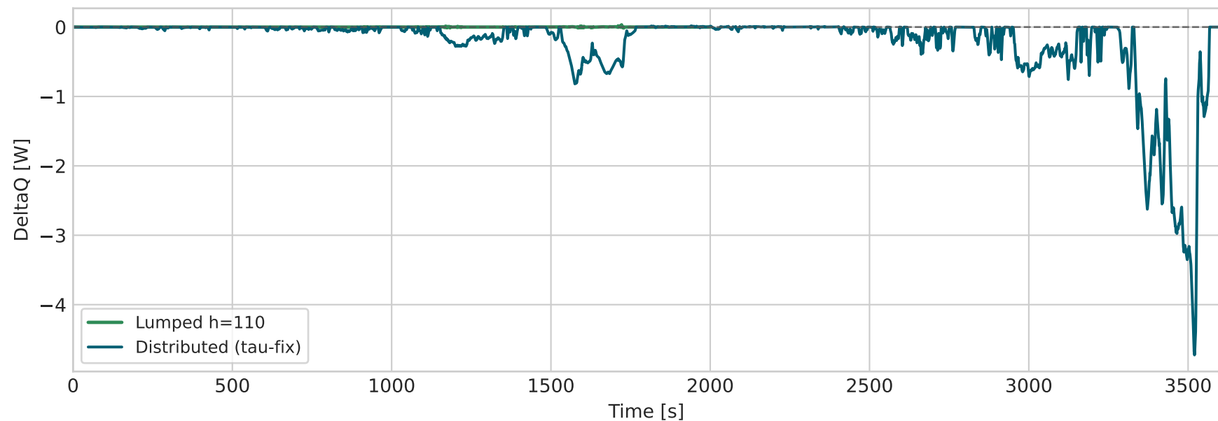
Heat Generation Error: Model - Validation
