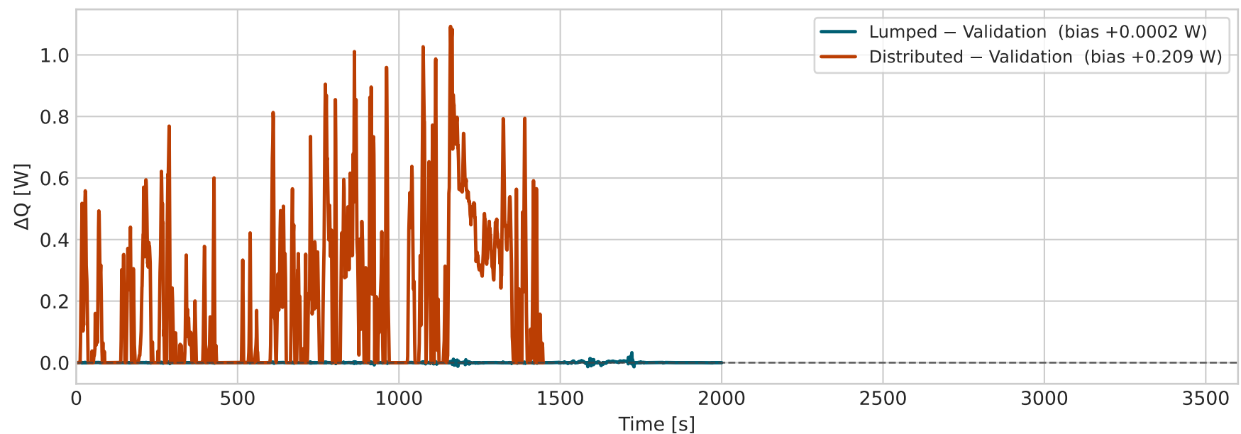
Heat Difference: Model – Validation
