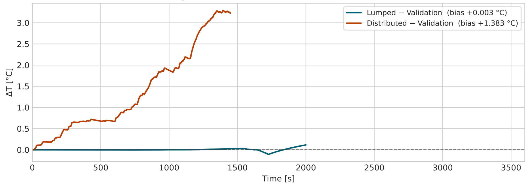
Temperature Difference: Model – Validation
