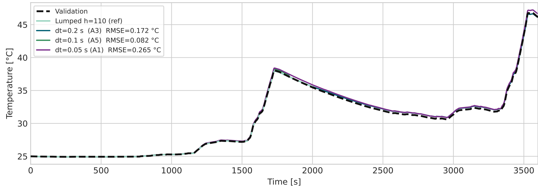
Temperature vs Validation — CFD dt sensitivity (N=1)
