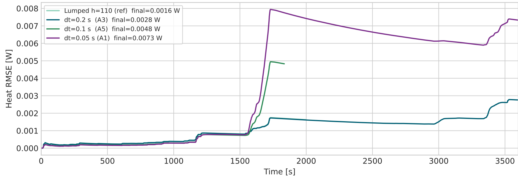
Running Heat Error RMS \sqrt{(\text{mean}(\Delta Q^2))} from t=0
