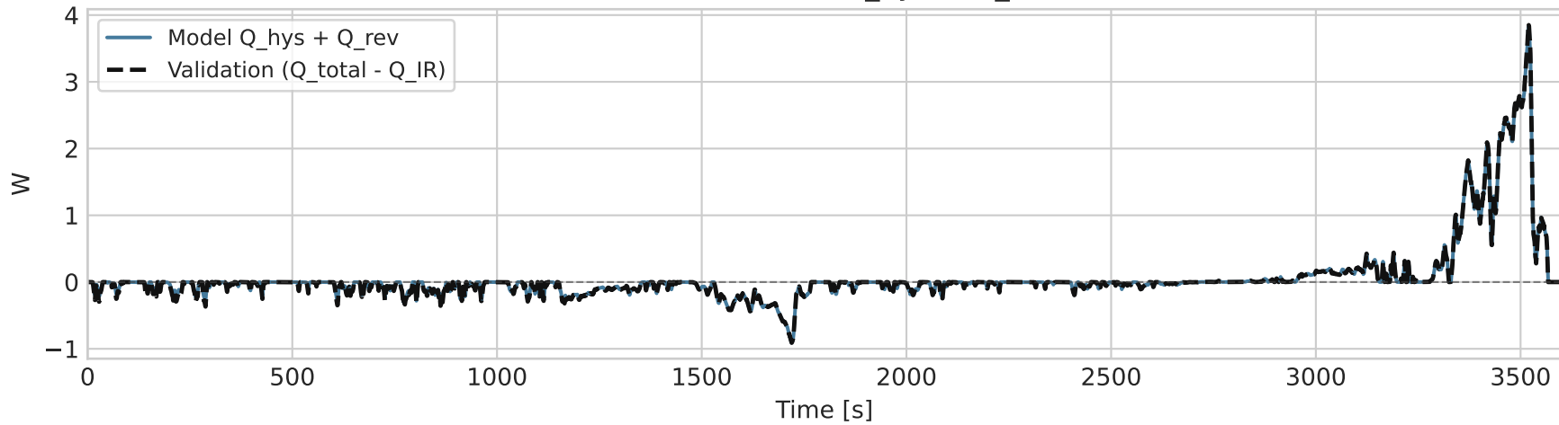
Non-ohmic heat: Q_hys + Q_rev
