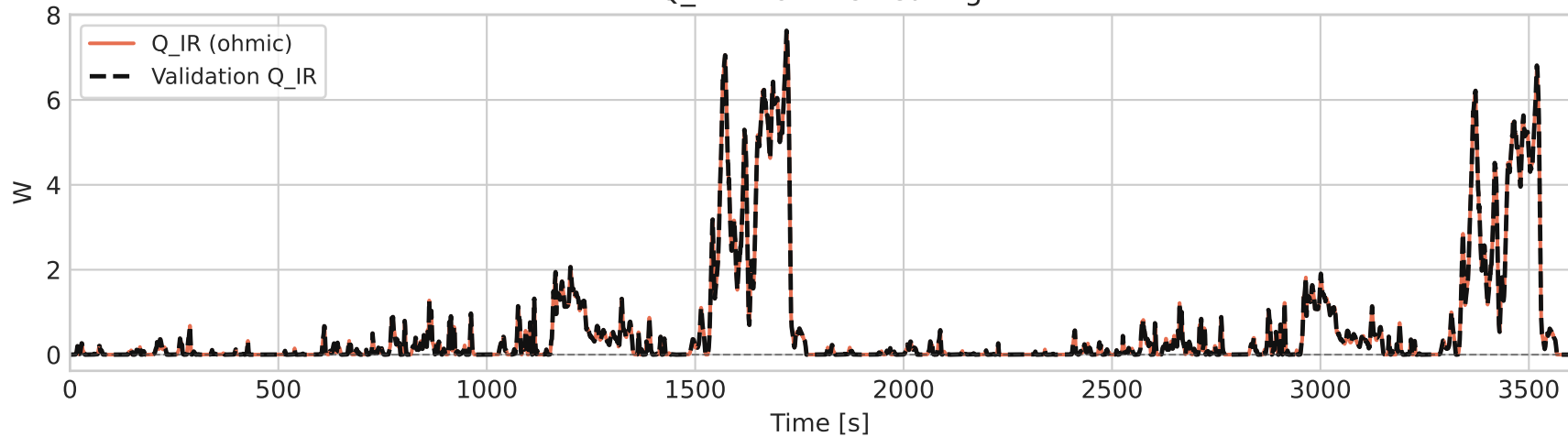
Q_IR — ohmic heating
