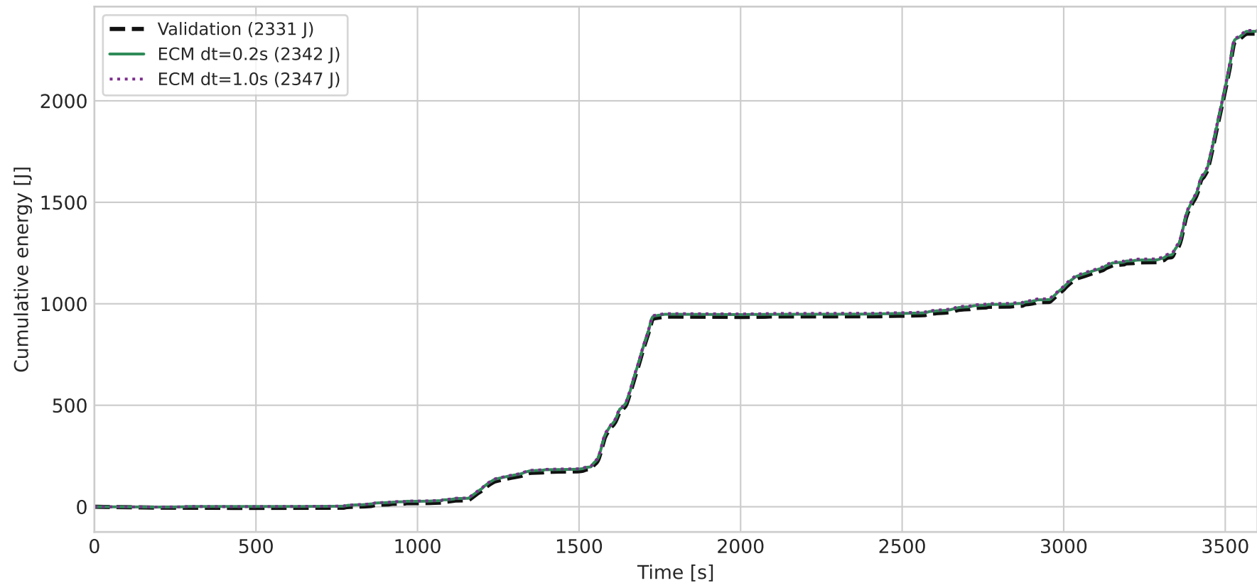
Cumulative energy: ECM vs Validation
