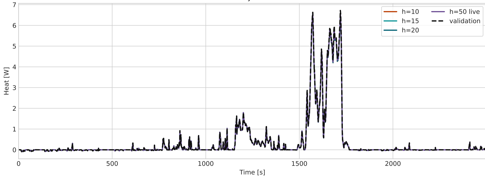
Heat Overlay vs Validation
