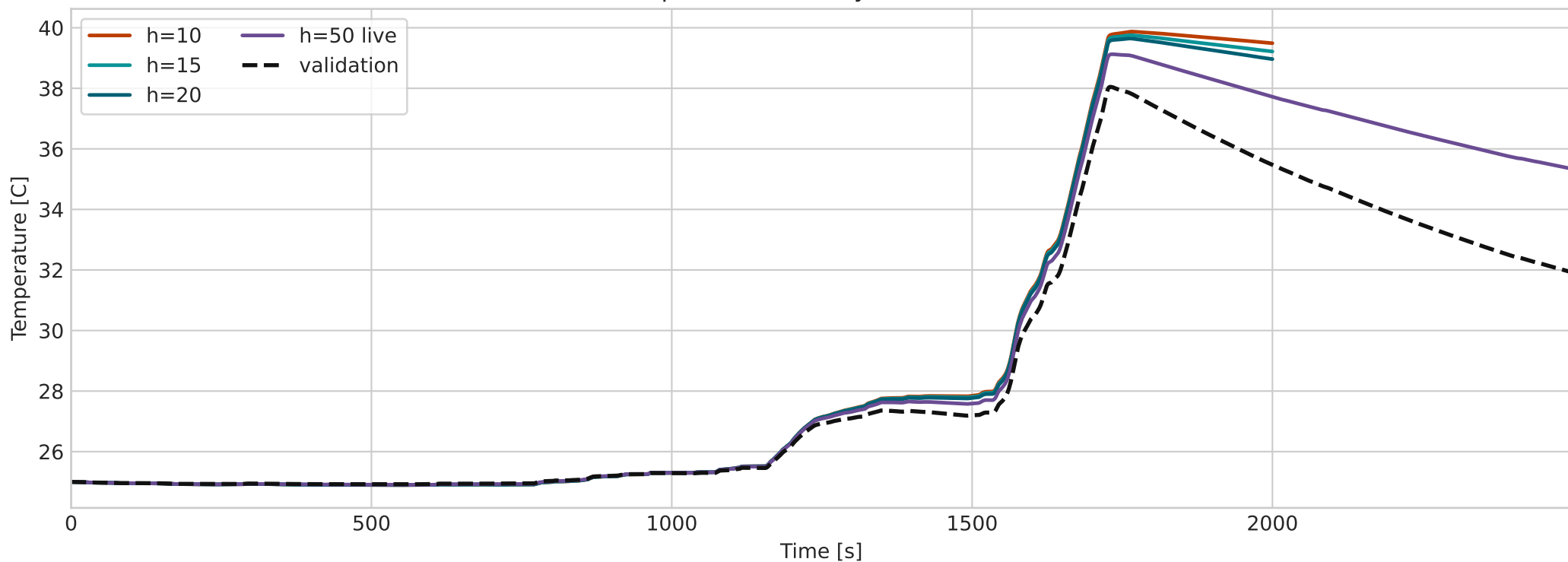
Heat Overlay vs Validation
