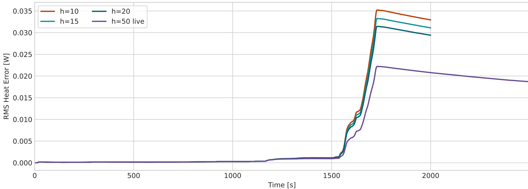
Running RMS Heat Error vs Validation
