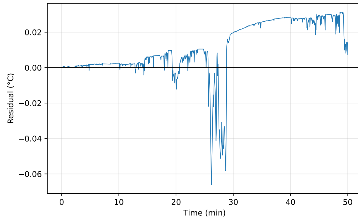
Residuals — fitted model (RMSE = 0.0186 ^{\circ}\text{C} )
