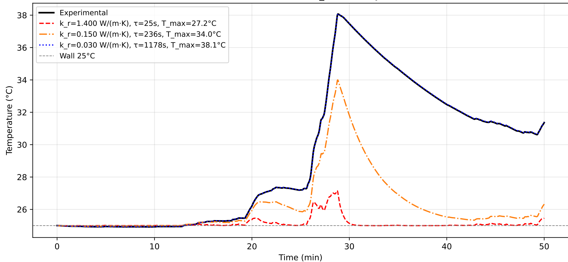
1D radial model — k_r sensitivity
