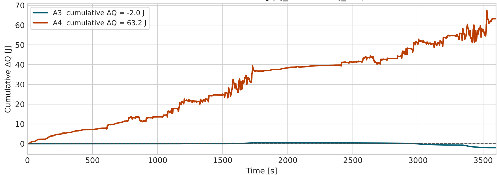
Cumulative Heat Error \int(Q_{\text{model}} - Q_{\text{val}}) dt
