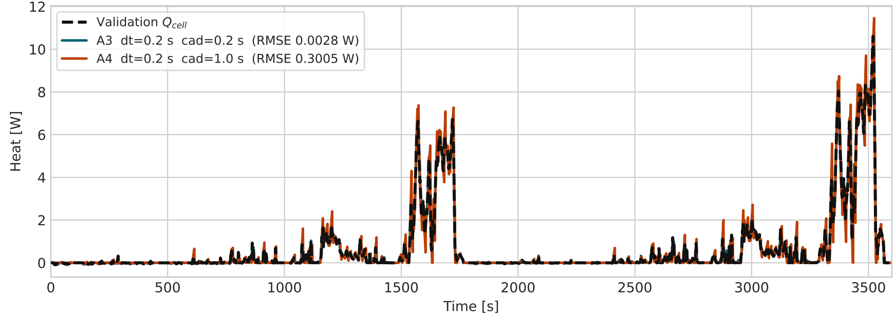
ECM Heat Generation vs Validation
