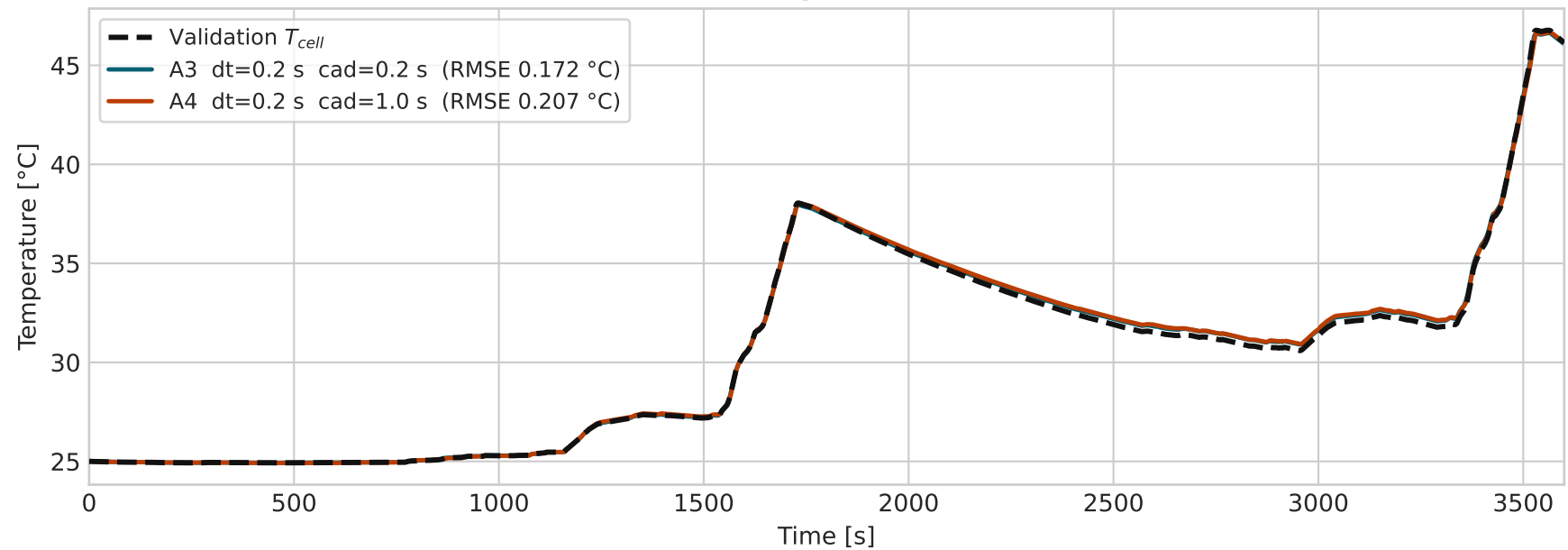
ECM Feedback Temperature vs Validation
