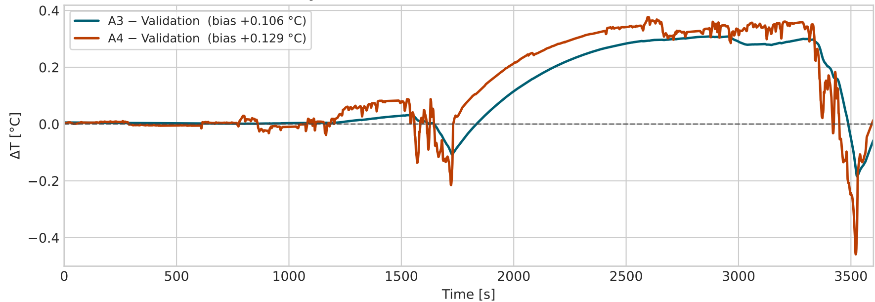
Temperature Difference: Model – Validation
