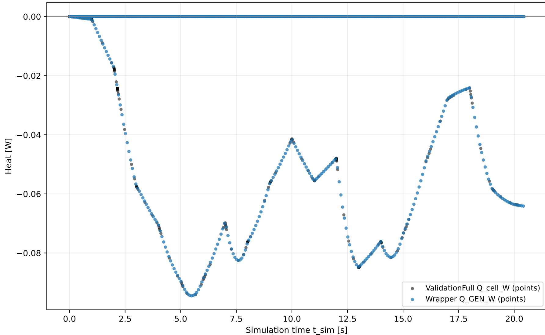
Points-only Heat Comparison (validationFull, clipped to solver max time)
