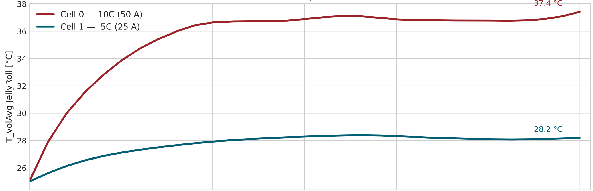
Two-Cell Test: Cell 0 (10C / 50 A) vs Cell 1 (5C / 25 A) parallelBranches ECM · dirKfix thermal BCs · thermally independent
