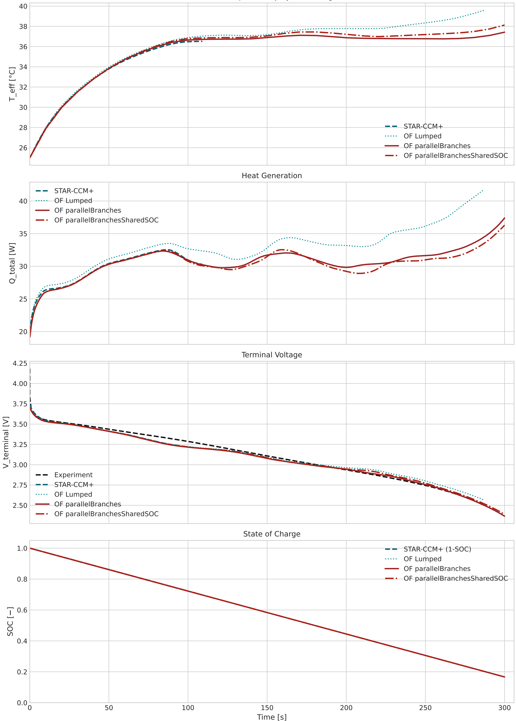
10C Discharge — parallelBranches vs parallelBranchesSharedSOC dirKfix BCs (directionalSolidThermo + contact-R split R/2) Cell Temperature (JellyRoll vol-avg)
