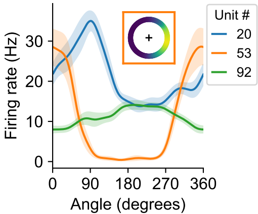
FEF tuning curves
