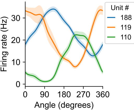
DMFC tuning curves
