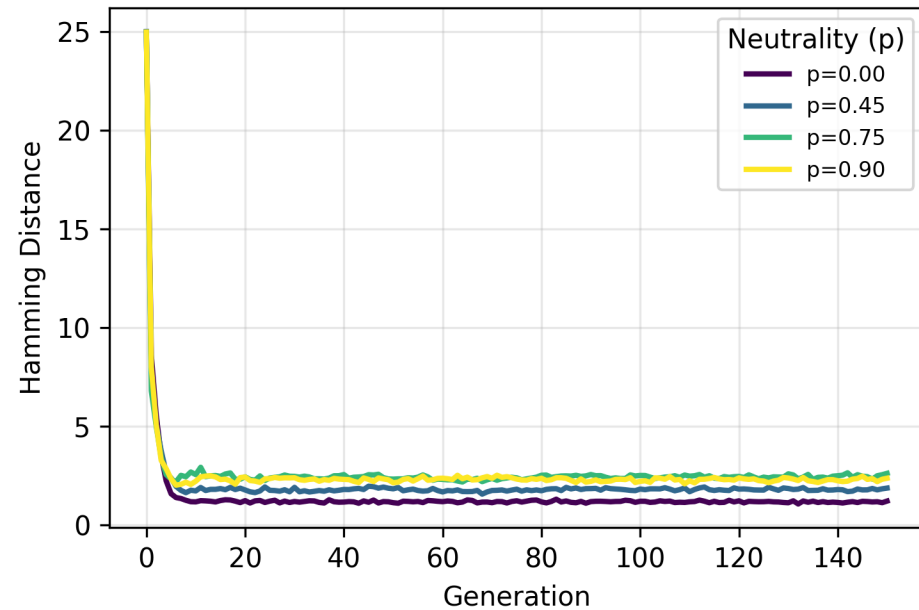
Hamming Distance Dynamics
