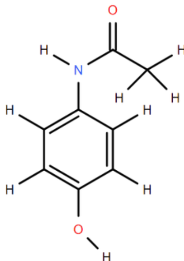
LEWIS STRUCTURE
