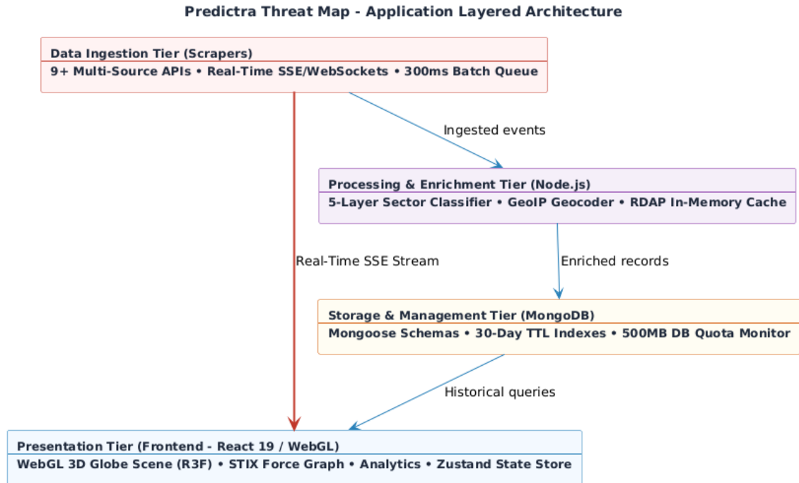
Figure 2.4: Predictra platform multi-tier layered application architecture.
