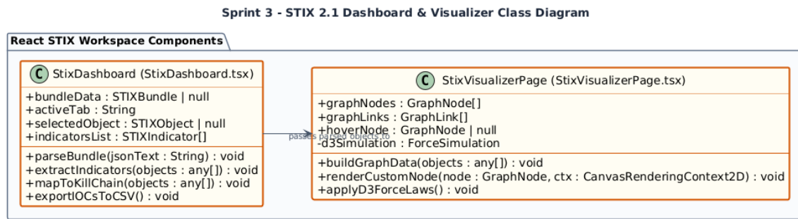
Figure 4.2: Sprint 3: Conception Class diagram.
