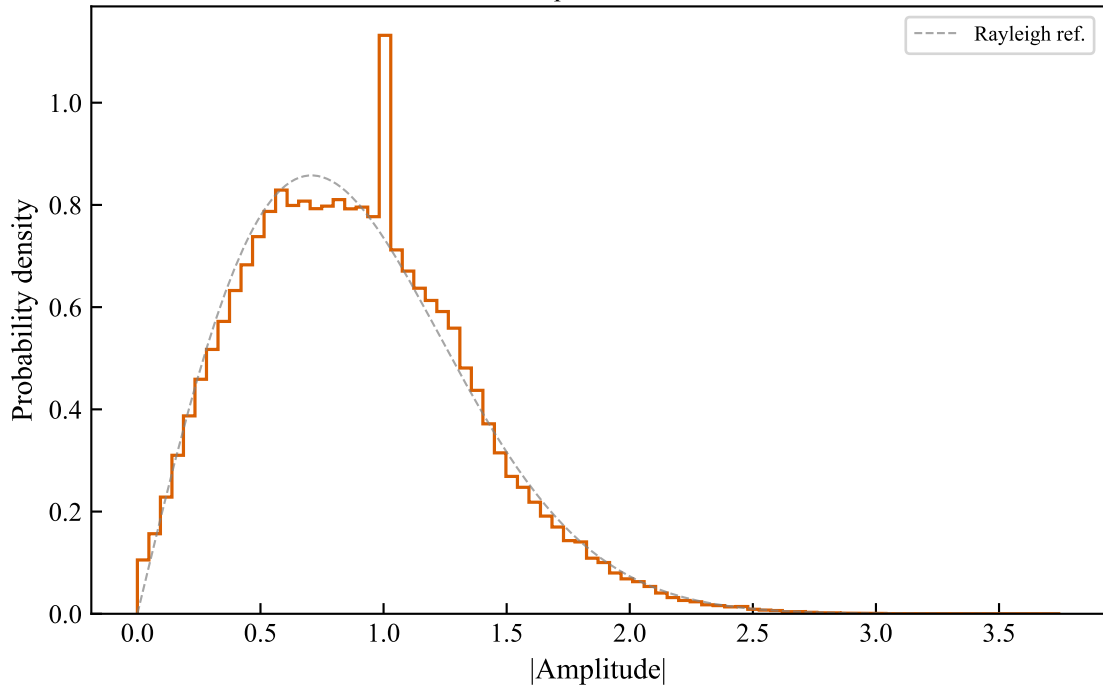
OFDM amplitude distribution
