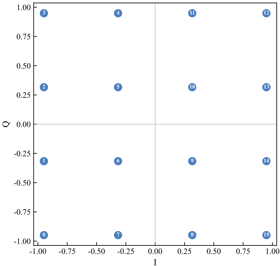
16QAM (16 points)
