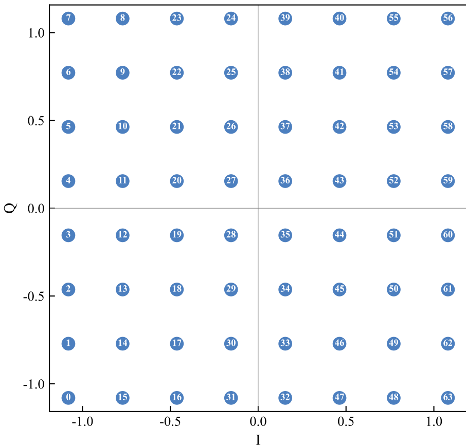
64QAM (64 points)
