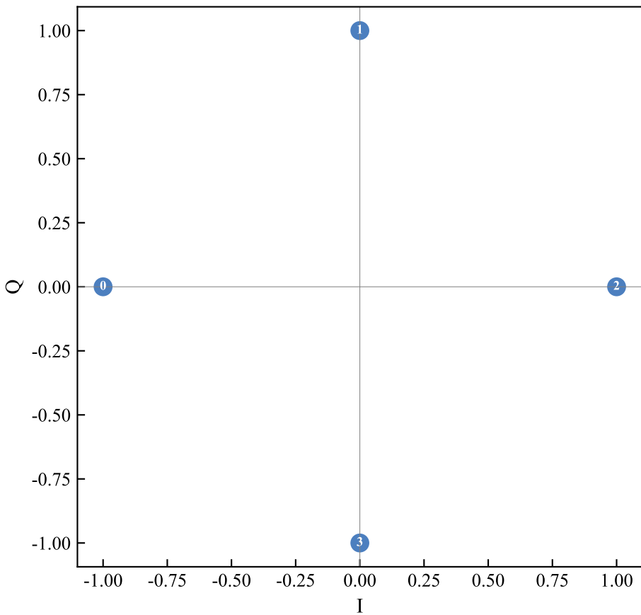
QPSK (4 points)
