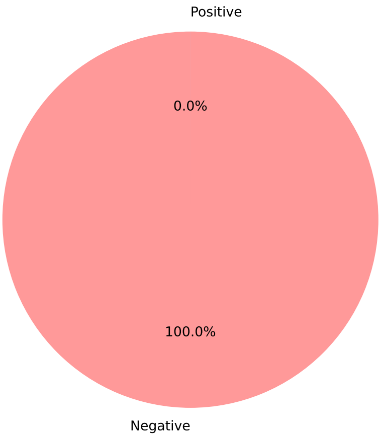
Class Distribution
