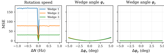
FIG. 5. Sensitivity of pattern MSE to single-parameter perturbations for a 3-prism (6-interface) system, plotted separately for rotation speed ( N , left), wedge angle \alpha_x (center), and wedge angle \alpha_y (right). Each curve represents one prism. Speed sensitivity exceeds \alpha_x by \sim 10^3 and \alpha_y by \sim 10^5 , explaining the error hierarchy in the final results.
