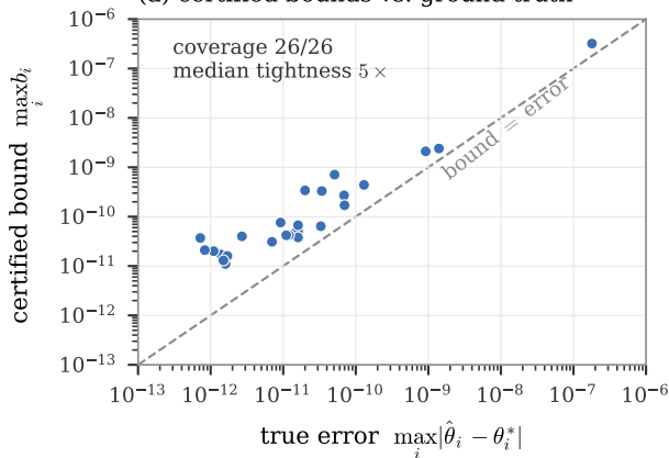
(a) certified bounds vs. ground truth
