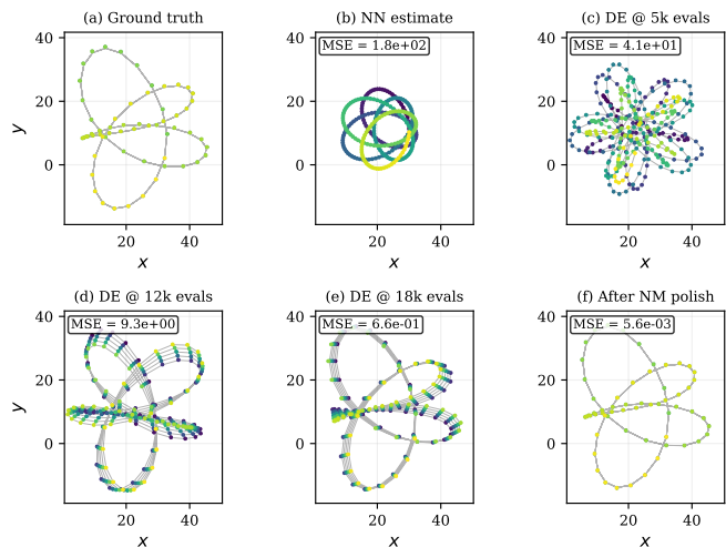
FIG. 6. Convergence for a 3-prism system: (a) ground truth, (b) coarse initial estimate, (c–e) DE snapshots at 5k, 12k, 18k evaluations, (f) after NM polish ( \text{MSE} \sim 10^{-3} ).
