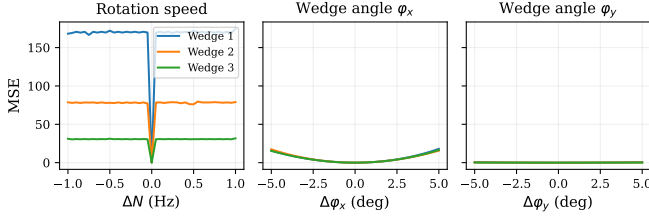
FIG. 5. Sensitivity of pattern MSE to single-parameter perturbations for a 3-prism (6-interface) system, plotted separately for rotation speed ( N , left), wedge angle \alpha_x ( \alpha_x , centre), and wedge angle \alpha_y ( \alpha_y , right). Each curve represents one prism. Speed sensitivity exceeds \alpha_x by \sim 10^3 and \alpha_y by \sim 10^5 , explaining the error hierarchy in the final results.
