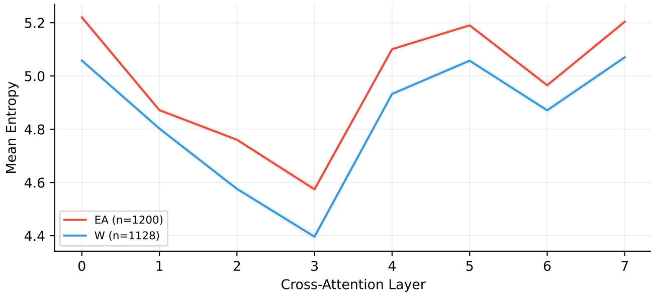
Llama Cross-Attention Entropy (peak d=+1.44 at L2)
