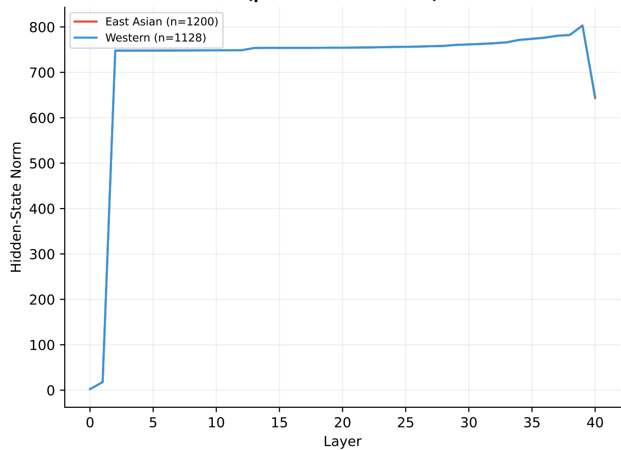
Llama: Hidden-State Norms (peak d=+2.81 at L23)
