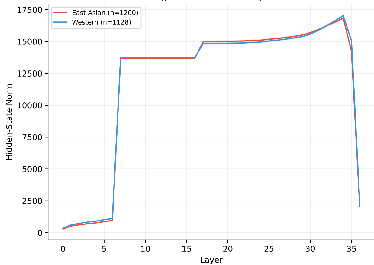
Qwen: Hidden-State Norms (peak d=-1.43 at L3)
