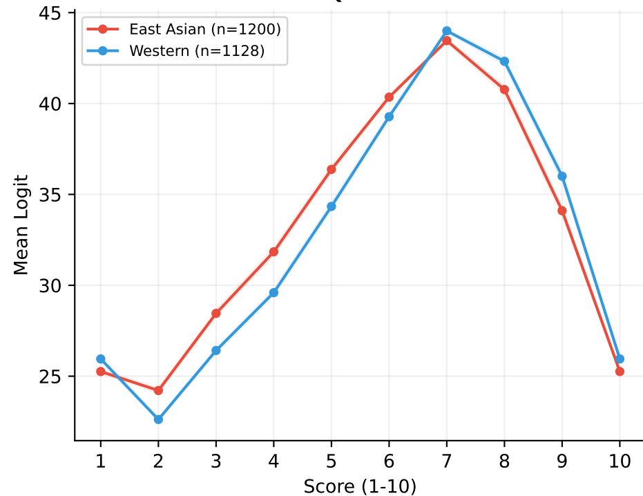
Qwen
