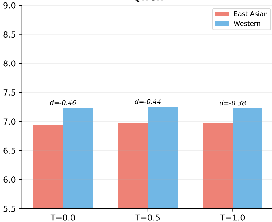
Qwen
