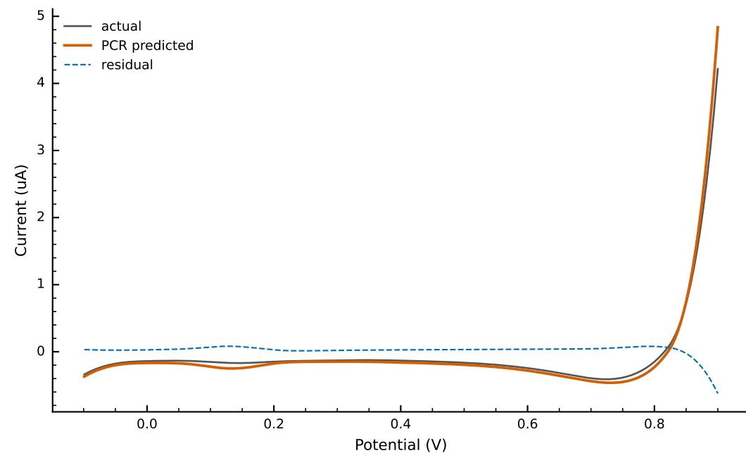
CV GC - Cathodic
