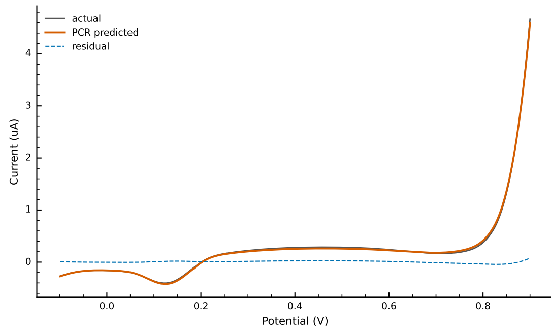
CV GC - Cathodic
