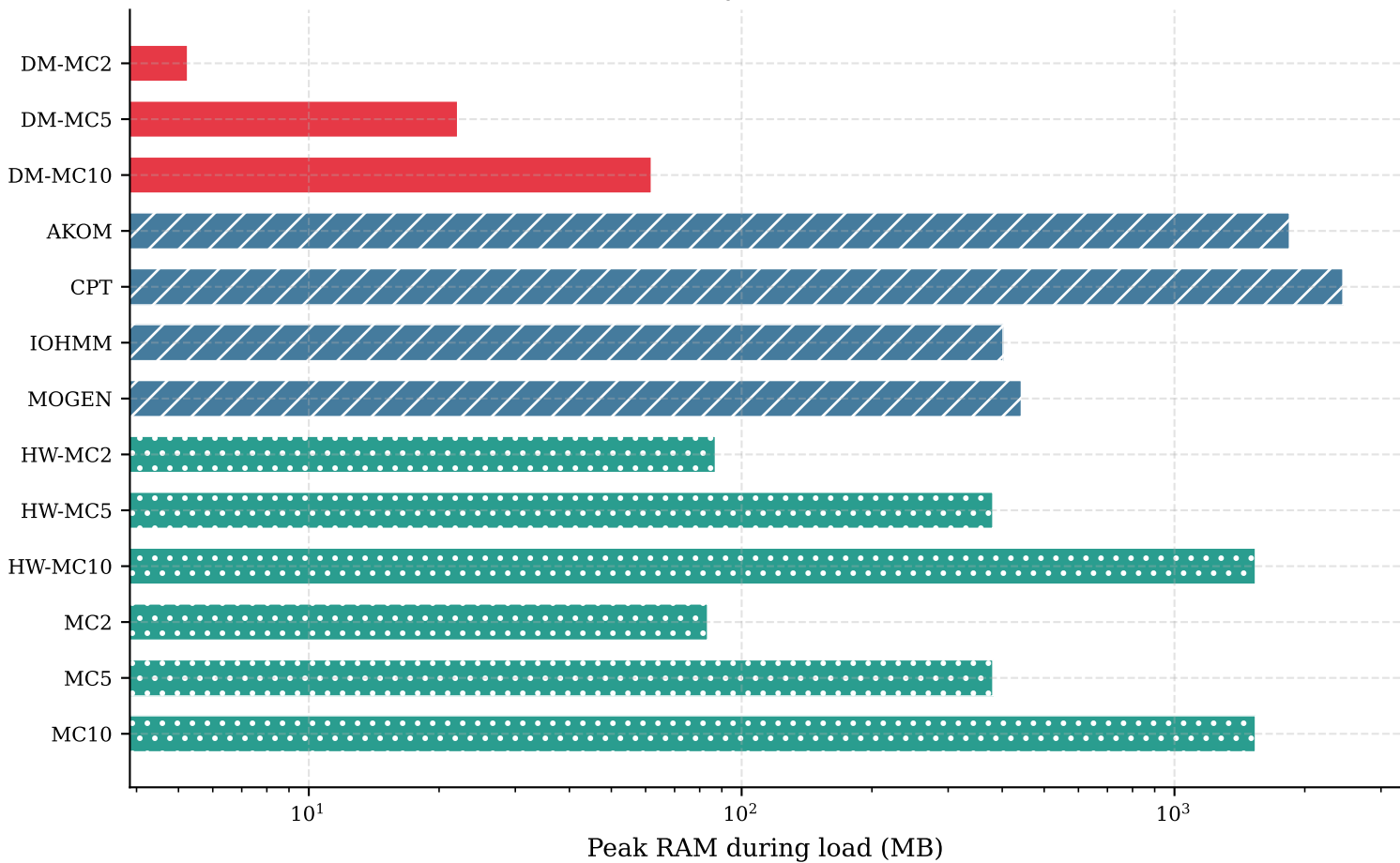
In-memory RAM footprint
