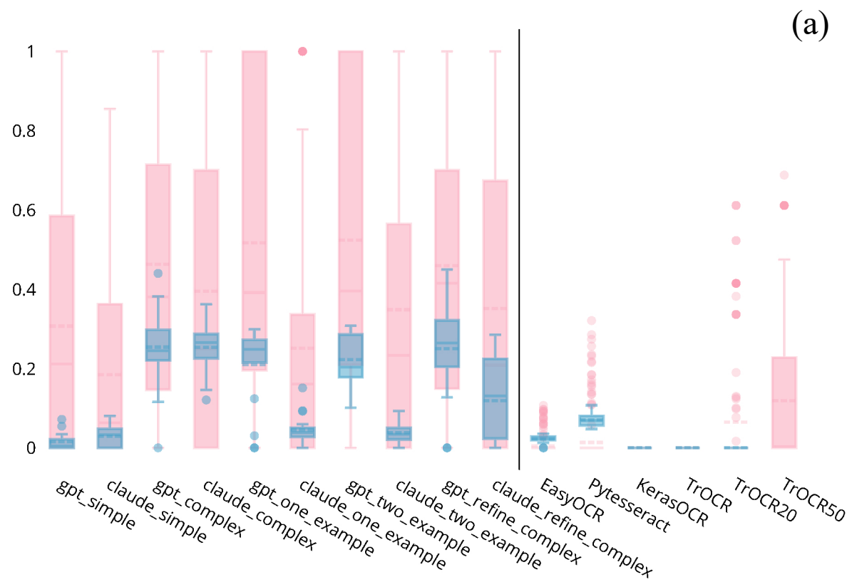
CER Score
