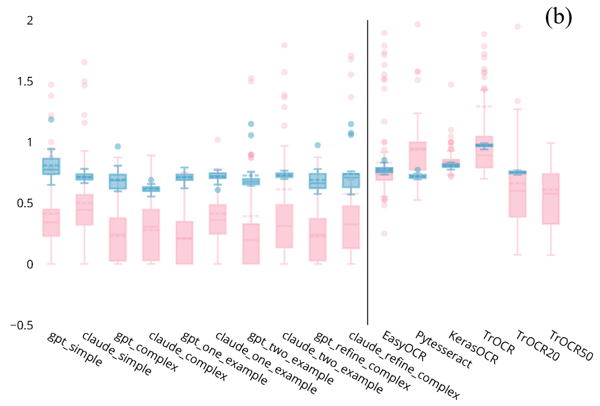
CER Score
