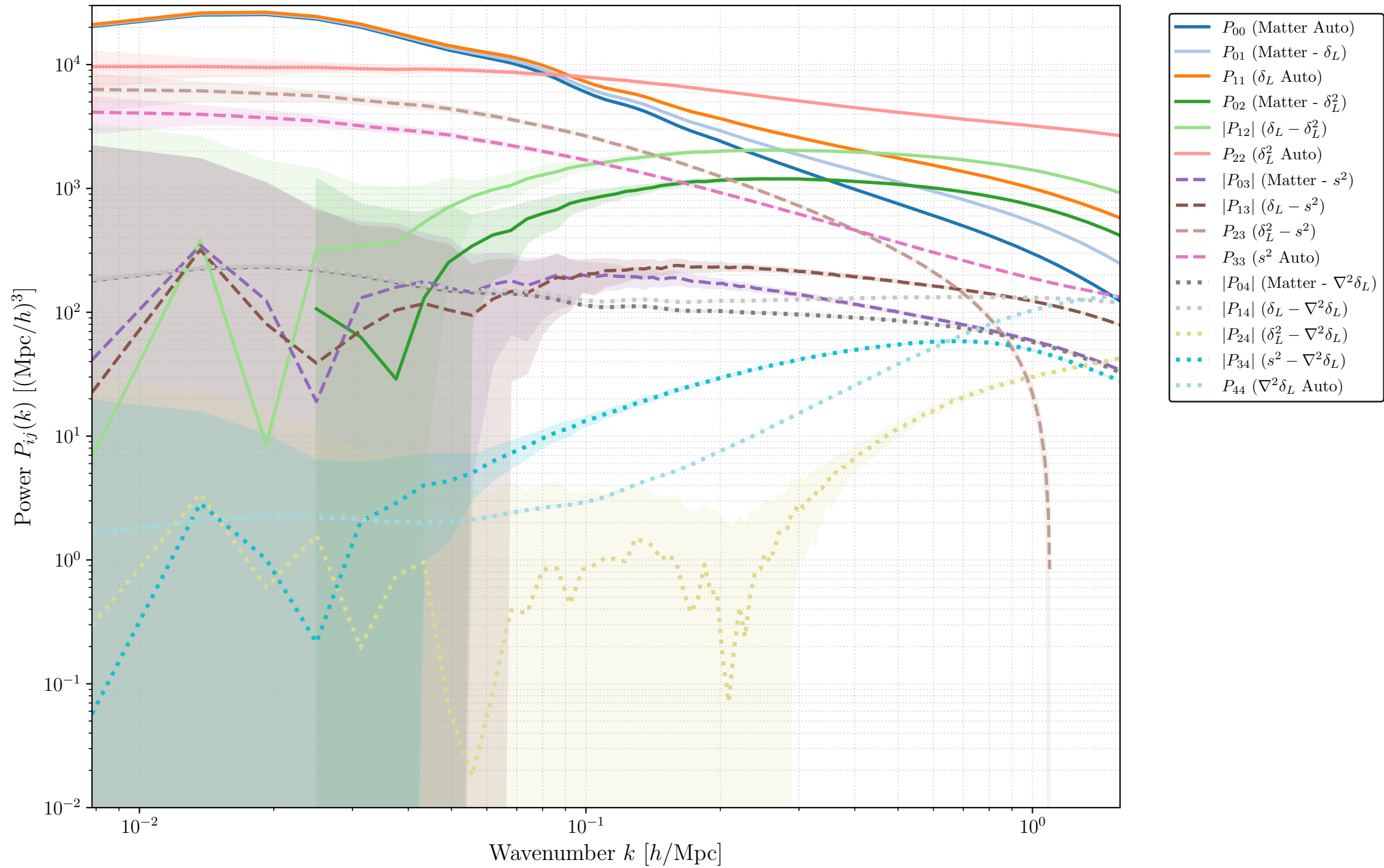
Ensemble Averaged Power Spectra with 1\sigma Variance ( N = 100 )
