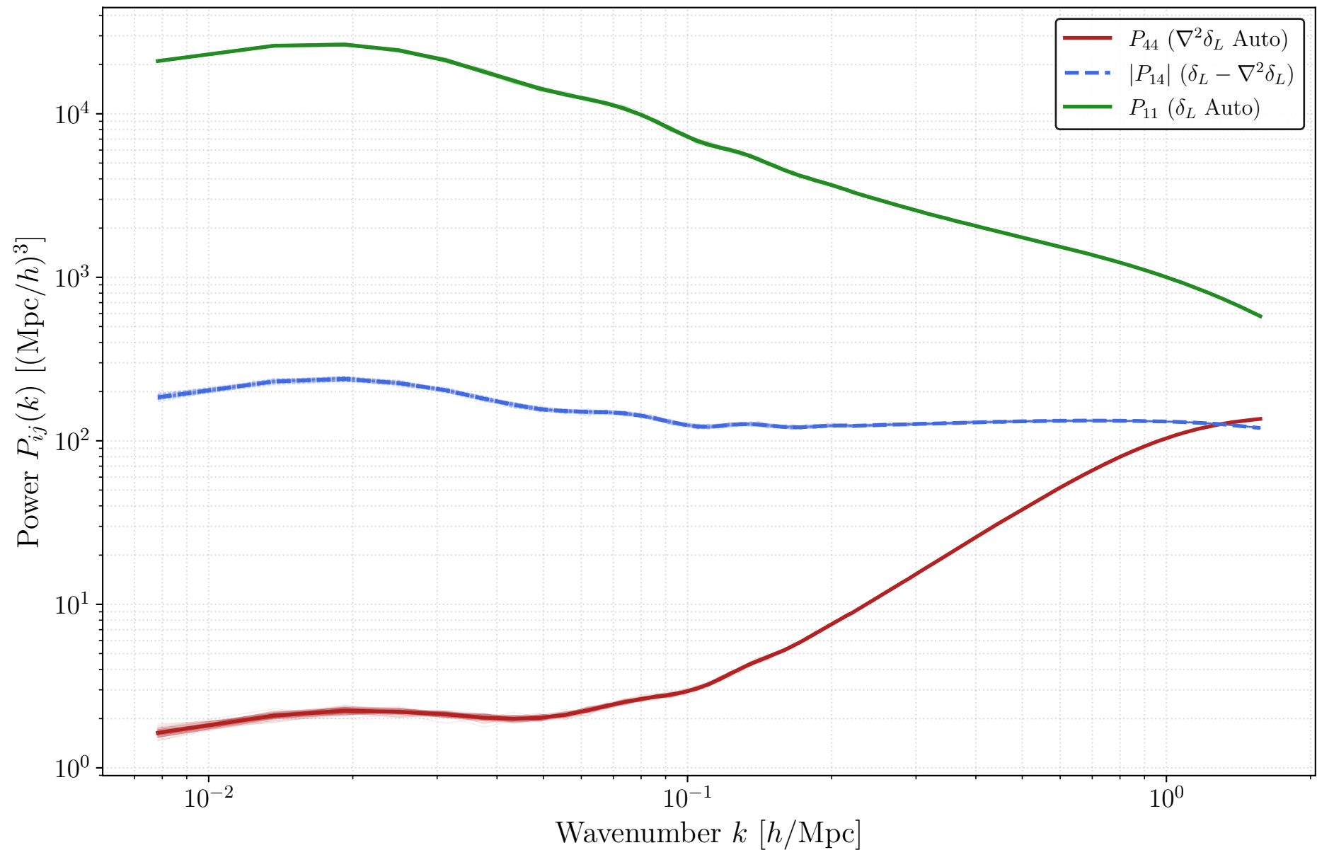
Ensemble Averaged Power Spectra ( N = 58 )
