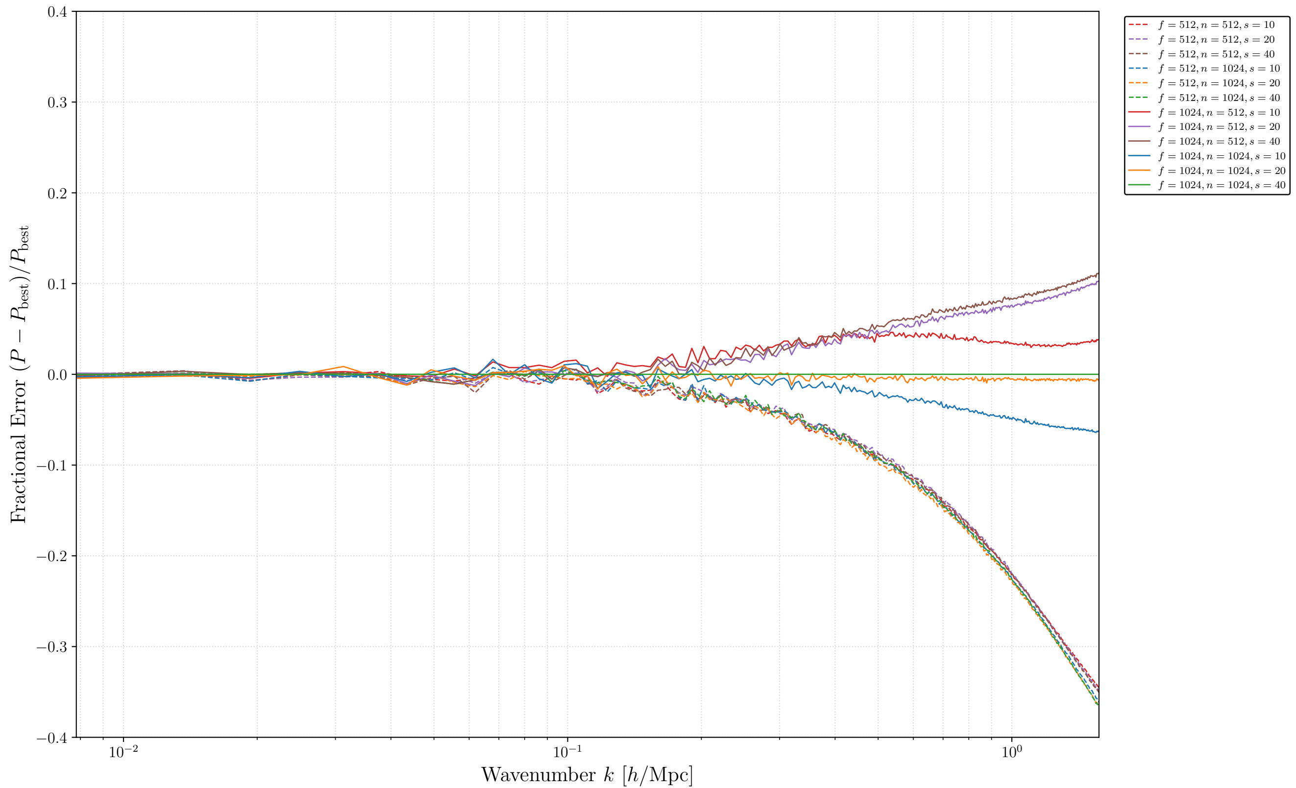
Fractional Error relative to Best (f1024, n1024, s40): P_{00} (Matter Auto)
