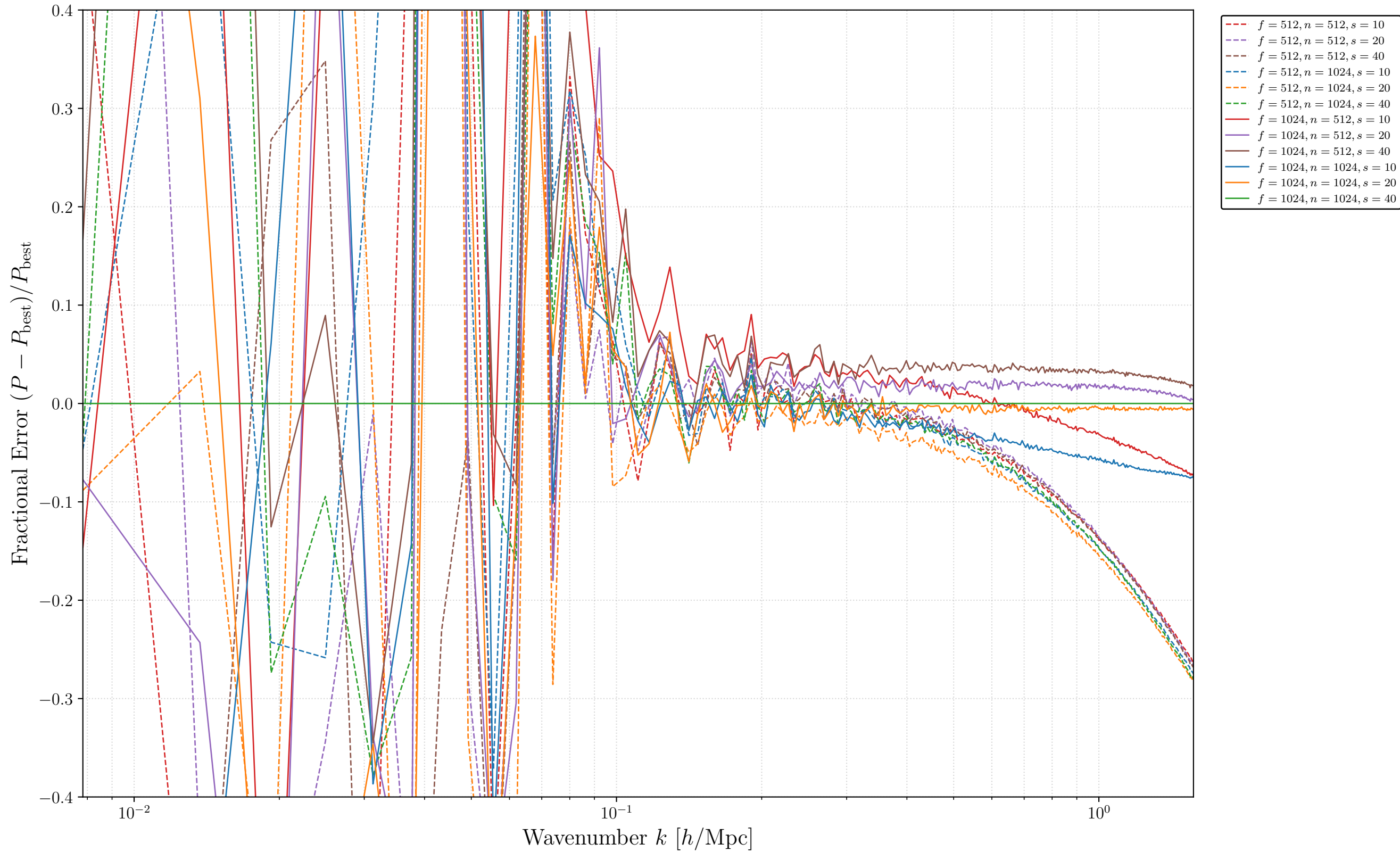
Fractional Error relative to Best (f1024, n1024, s40): P_{02} (Matter - \delta_L^2 )
