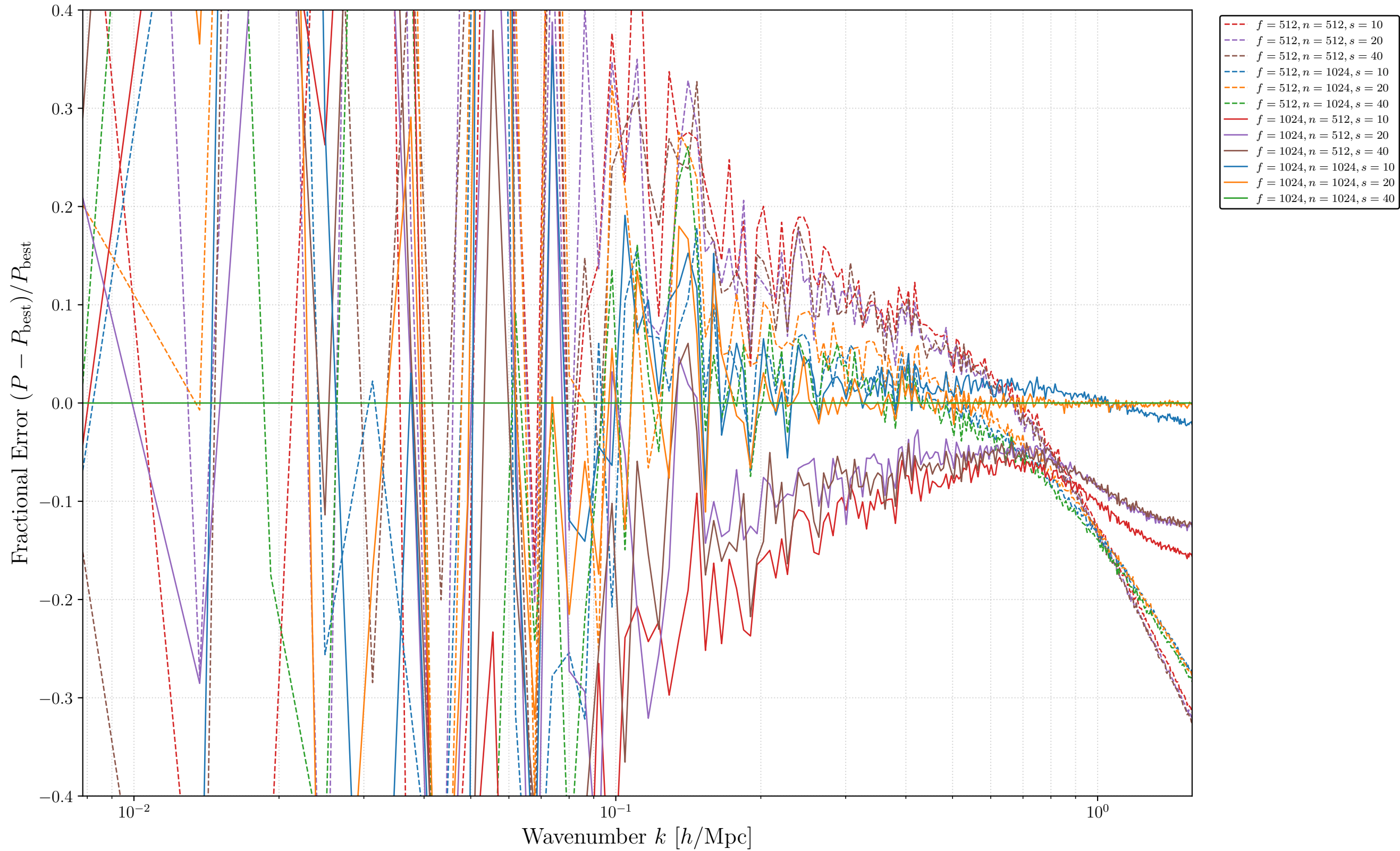
Fractional Error relative to Best (f1024, n1024, s40): |P_{03}| (Matter - s^2 )
