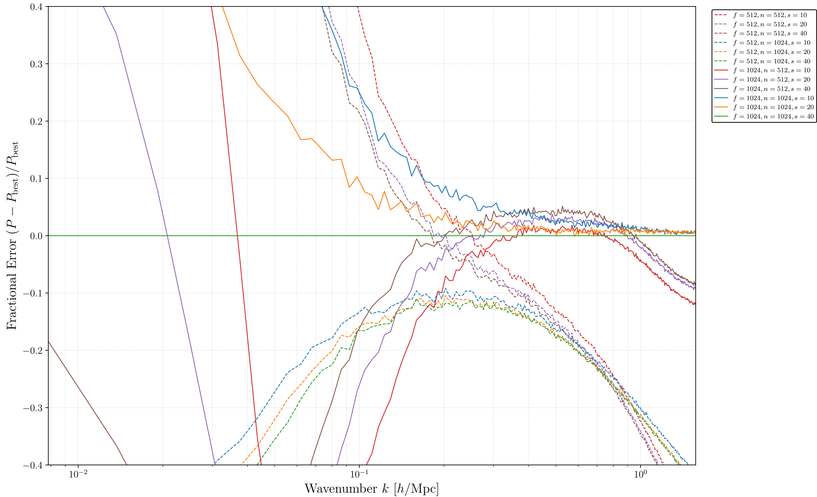
Fractional Error relative to Best (f1024, n1024, s40): |P_{04}| (Matter - \nabla^2\delta_L )
