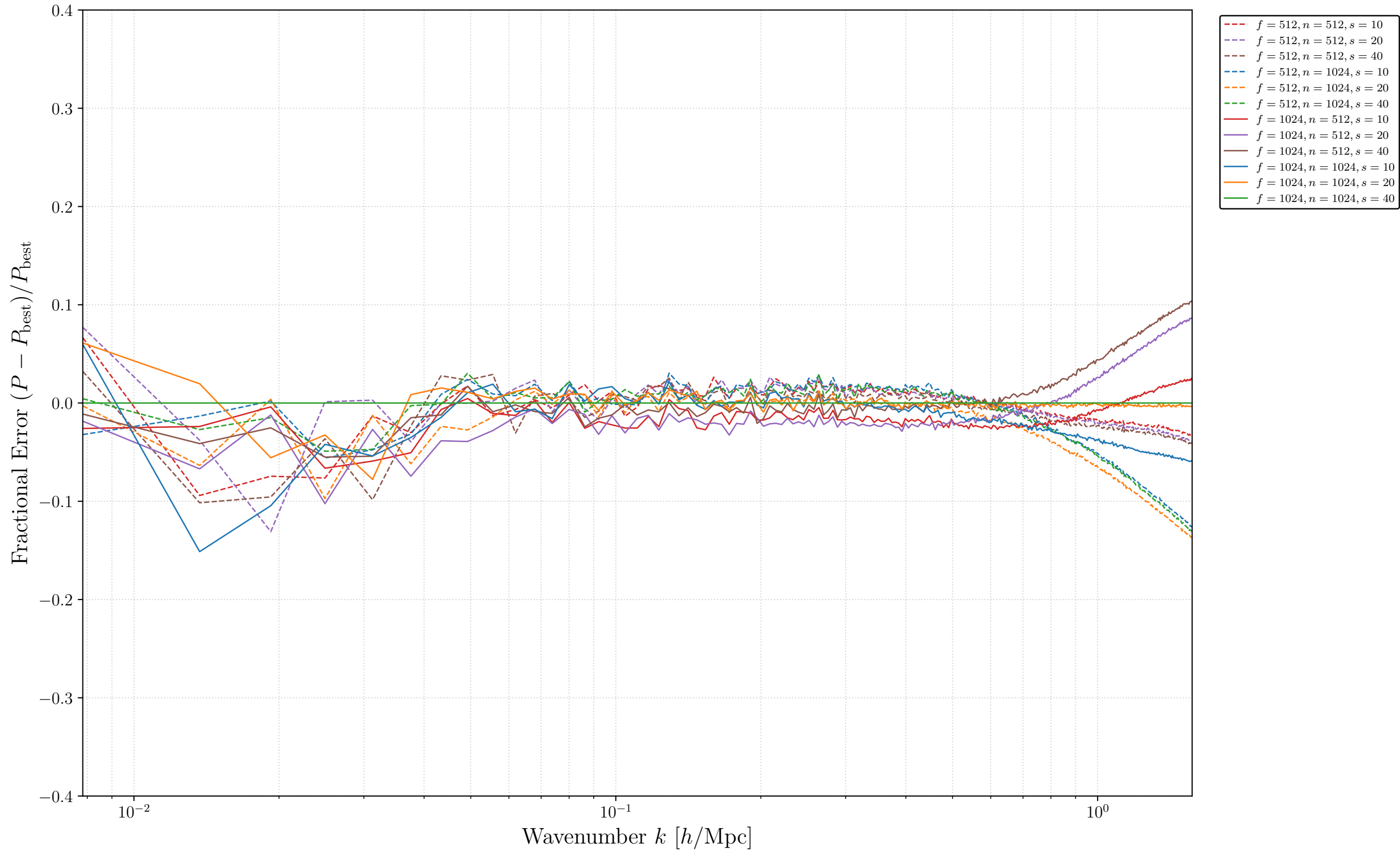
Fractional Error relative to Best (f1024, n1024, s40): P_{22} ( \delta_L^2 Auto)
