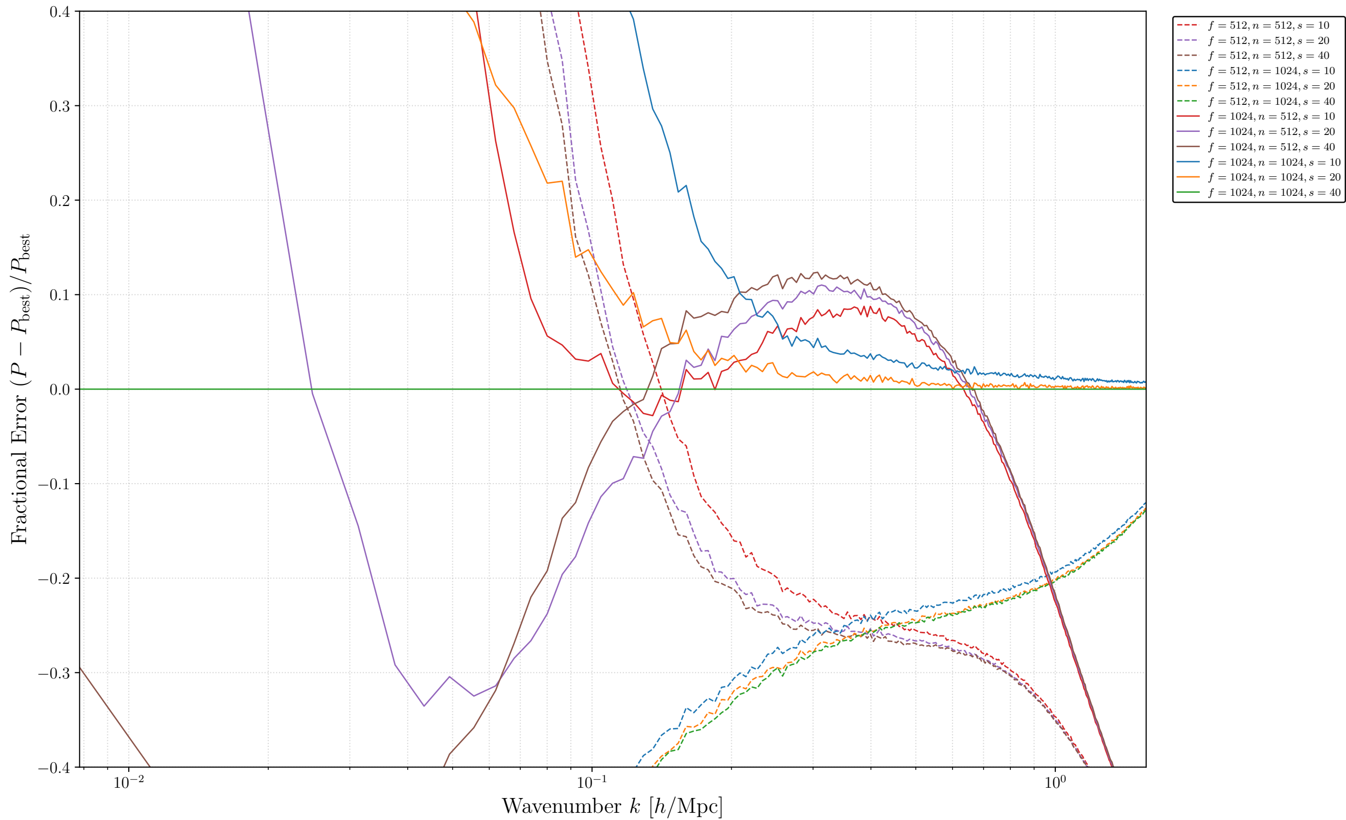
Fractional Error relative to Best (f1024, n1024, s40): P_{44} ( \nabla^2\delta_L Auto)
