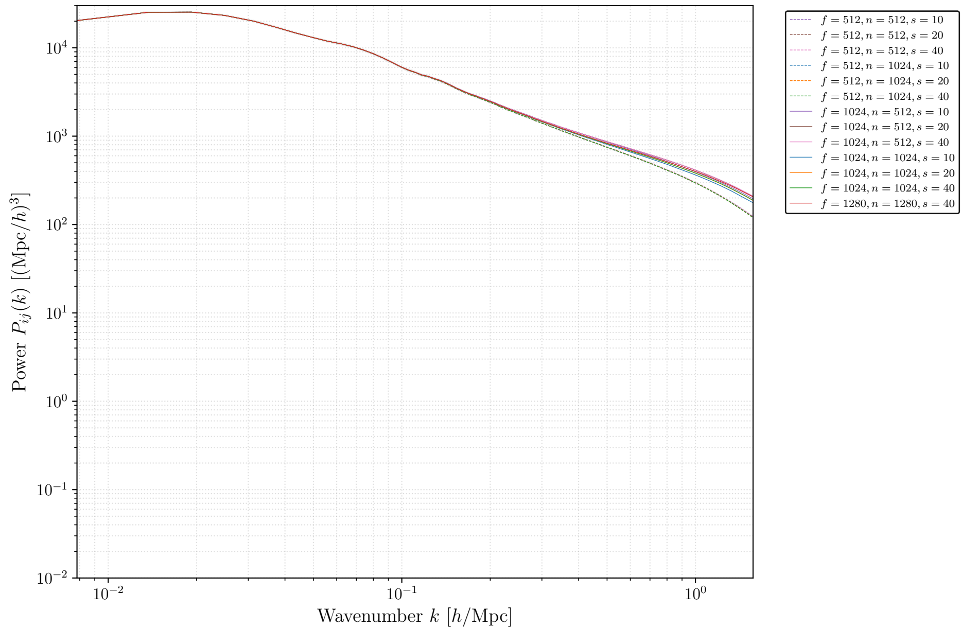
Spectrum P_{00} (Matter Auto) ( N = 10 versions)
