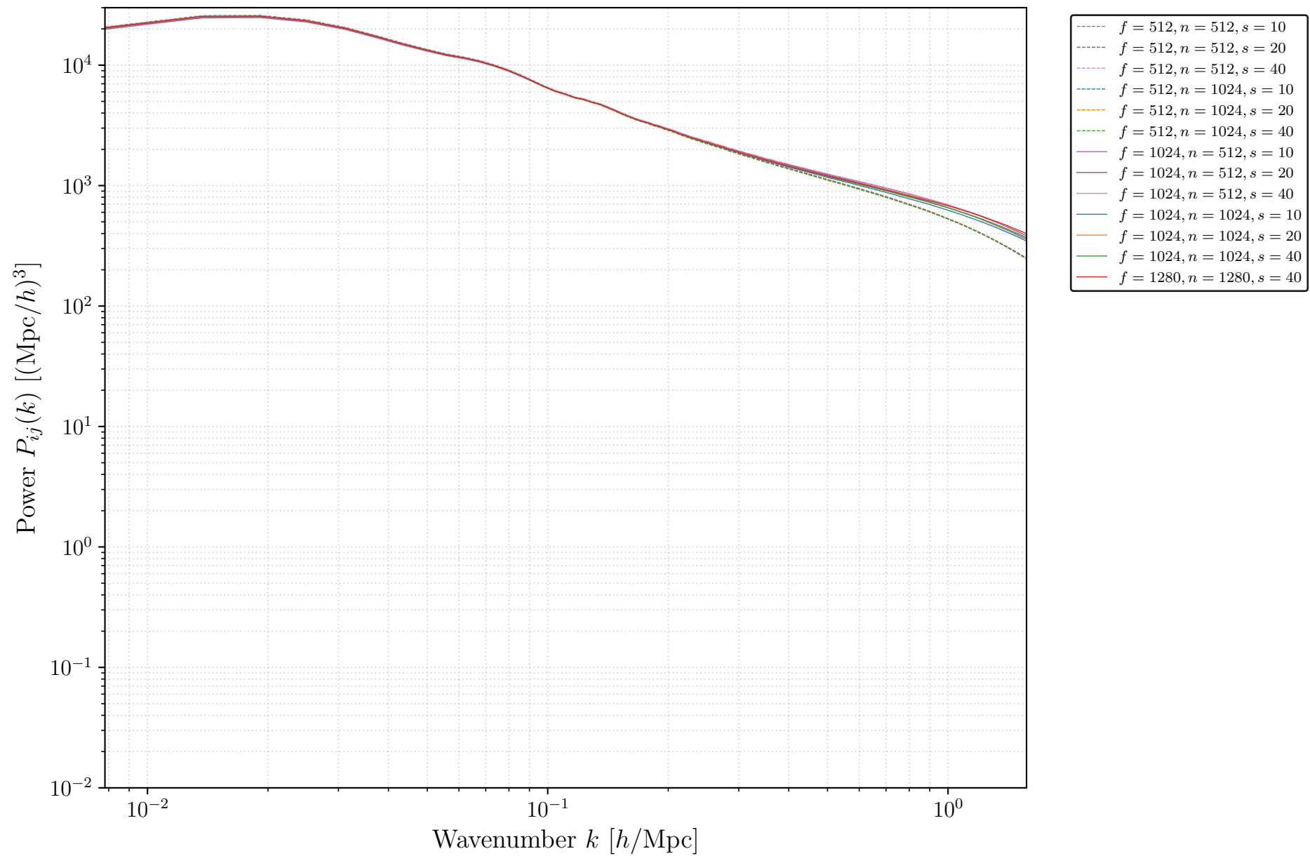
Spectrum P_{01} (Matter - \delta_L ) ( N = 10 versions)
