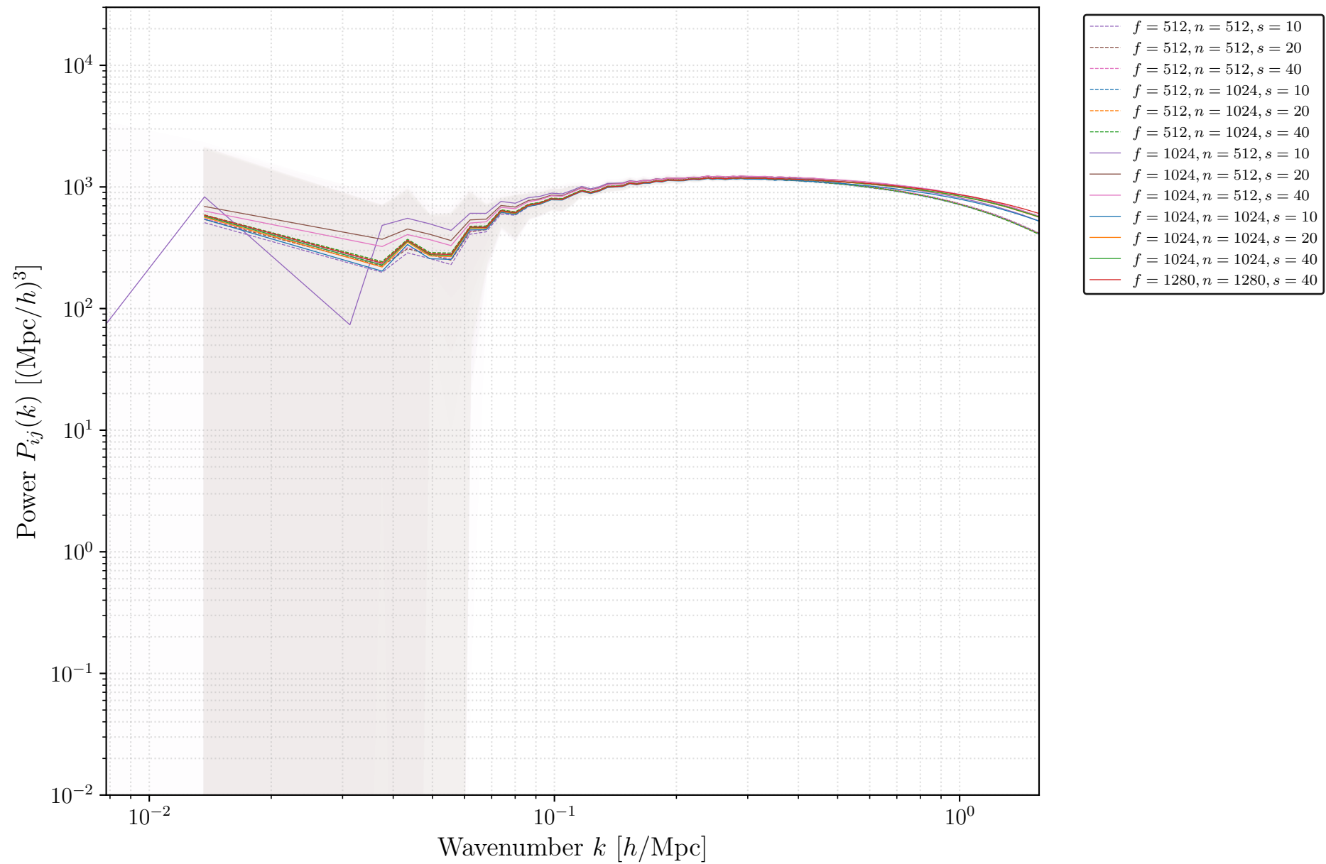
Spectrum P_{02} (Matter - \delta_L^2 ) ( N = 10 versions)
