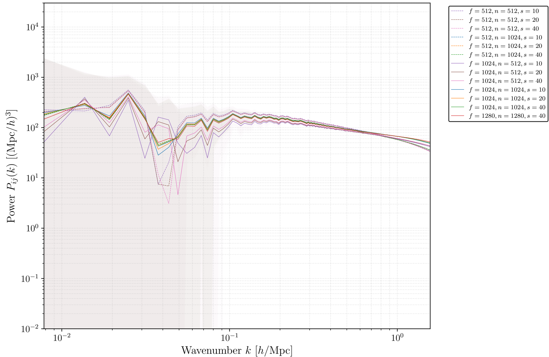
Spectrum |P_{03}| (Matter - s^2 ) ( N = 10 versions)
